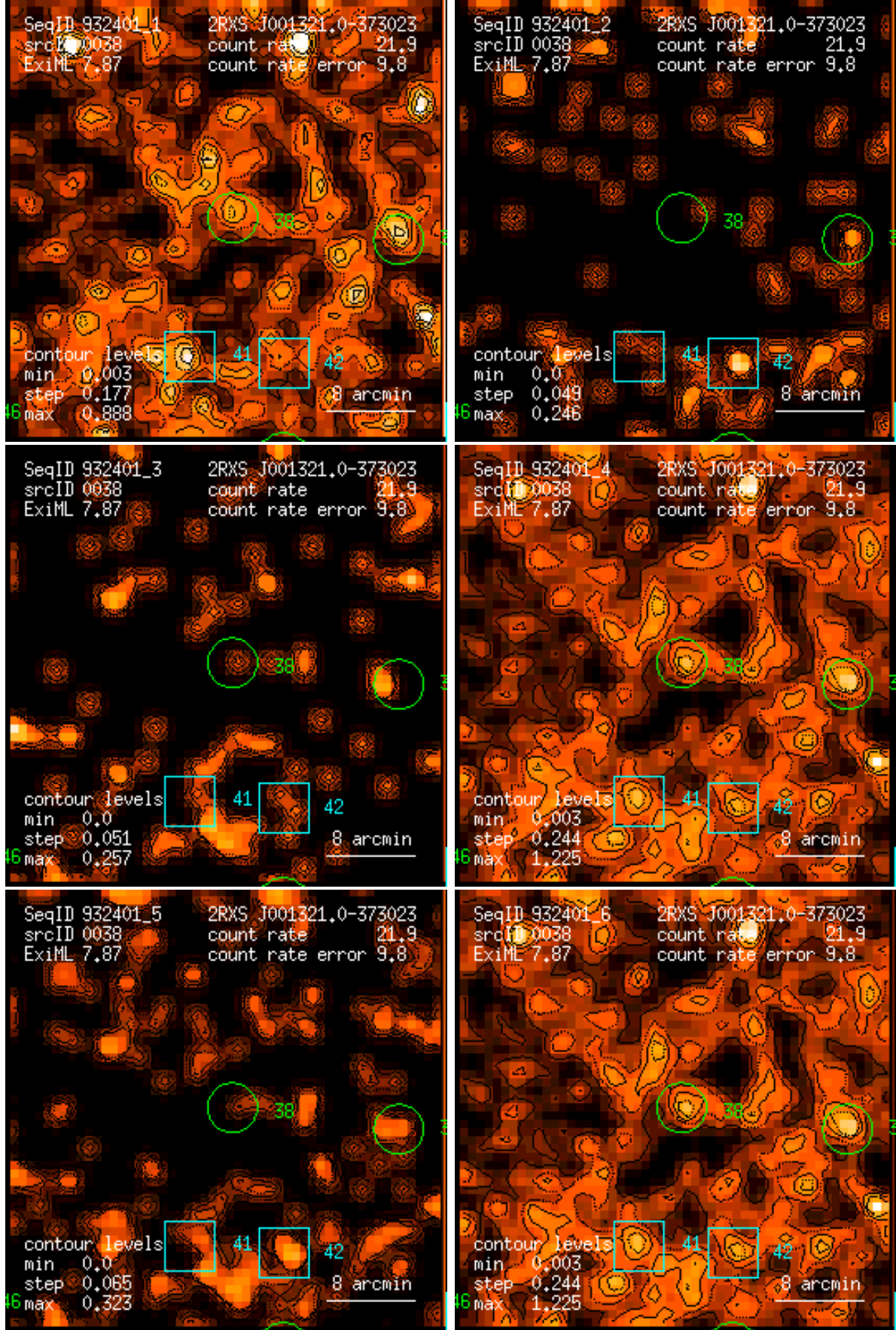
Figure 38: RASS 932401: detection 0038: band rate images, Gaussian filter: (1) PSPC channels 11 – 41, (2) 52 – 90, (3) 91 – 201, (4) 11 – 235, (5) 52 – 201, (6) 11 – 201. Broad band rates in counts/ks. Band rate contour levels in counts/ks/arcmin 2 .
