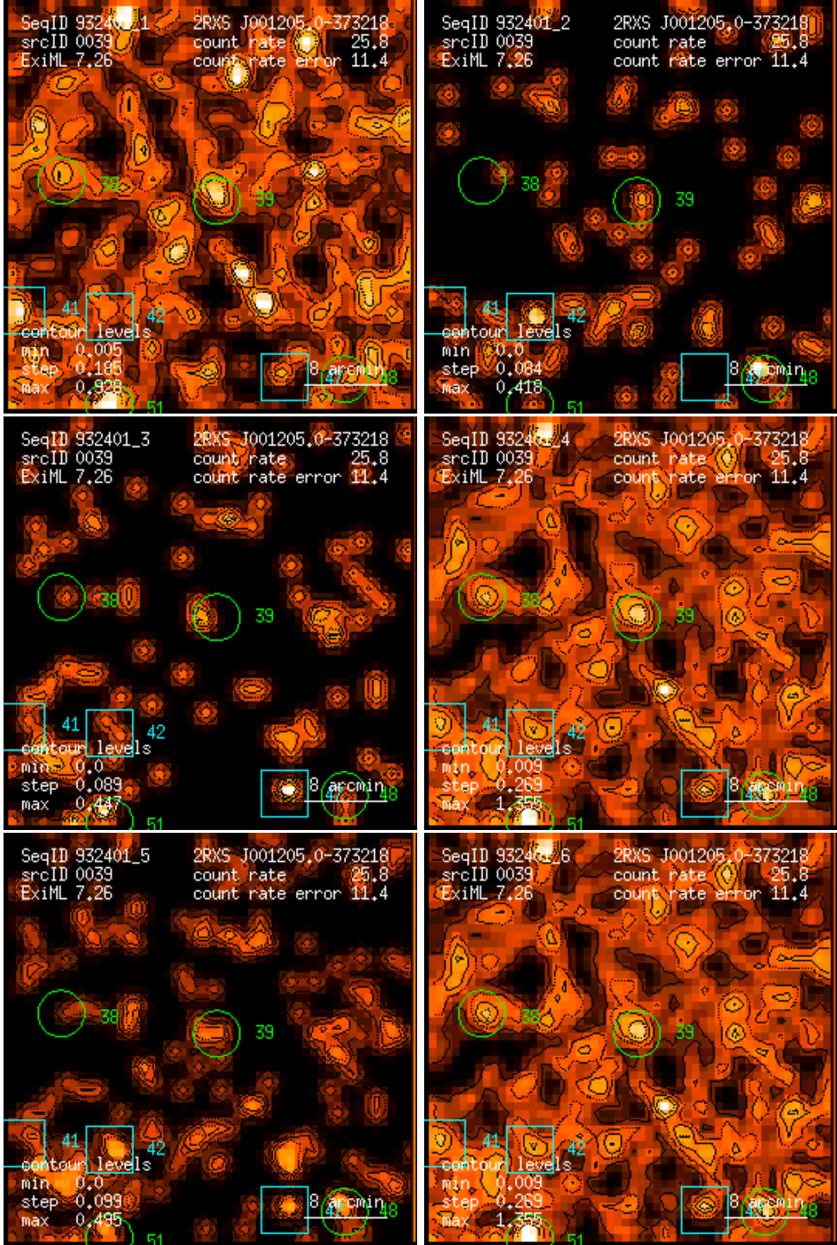
Figure 39: RASS 932401: detection 0039: band rate images, Gaussian filter: (1) PSPC channels 11 – 41, (2) 52 – 90, (3) 91 – 201, (4) 11 – 235, (5) 52 – 201, (6) 11 – 201. Broad band rates in counts/ks. Band rate contour levels in counts/ks/arcmin 2 .
