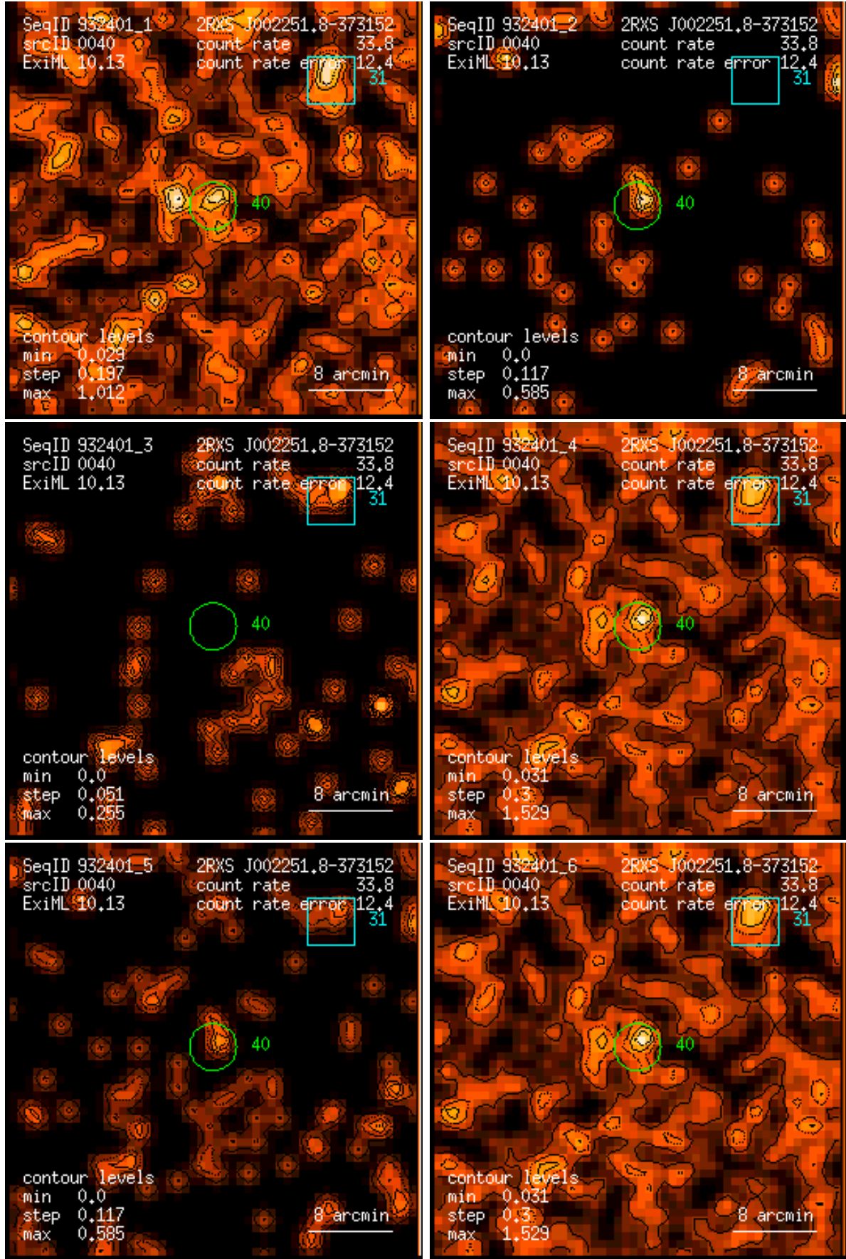
Figure 40: RASS 932401: detection 0040: band rate images, Gaussian filter: (1) PSPC channels 11 – 41, (2) 52 – 90, (3) 91 – 201, (4) 11 – 235, (5) 52 – 201, (6) 11 – 201. Broad band rates in counts/ks. Band rate contour levels in counts/ks/arcmin 2 .
