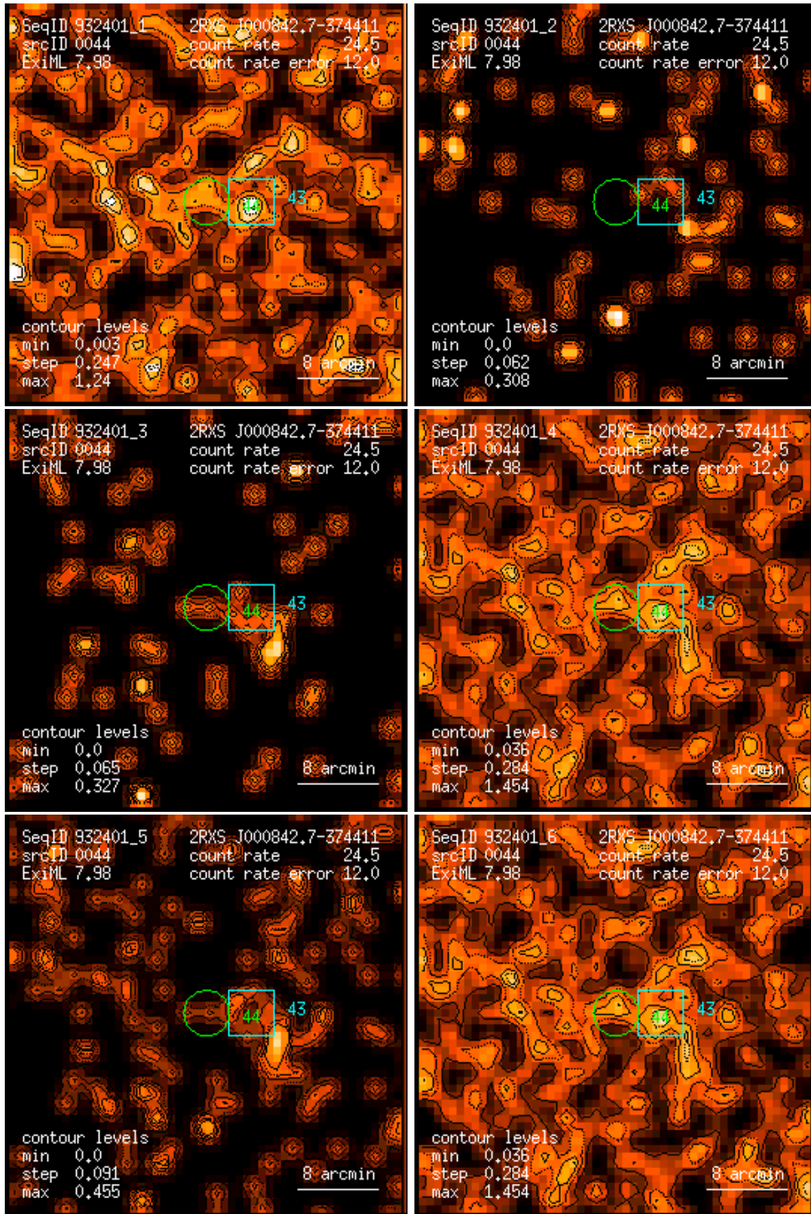
Figure 44: RASS 932401: detection 0044: band rate images, Gaussian filter: (1) PSPC channels 11 – 41, (2) 52 – 90, (3) 91 – 201, (4) 11 – 235, (5) 52 – 201, (6) 11 – 201. Broad band rates in counts/ks. Band rate contour levels in counts/ks/arcmin 2 .
