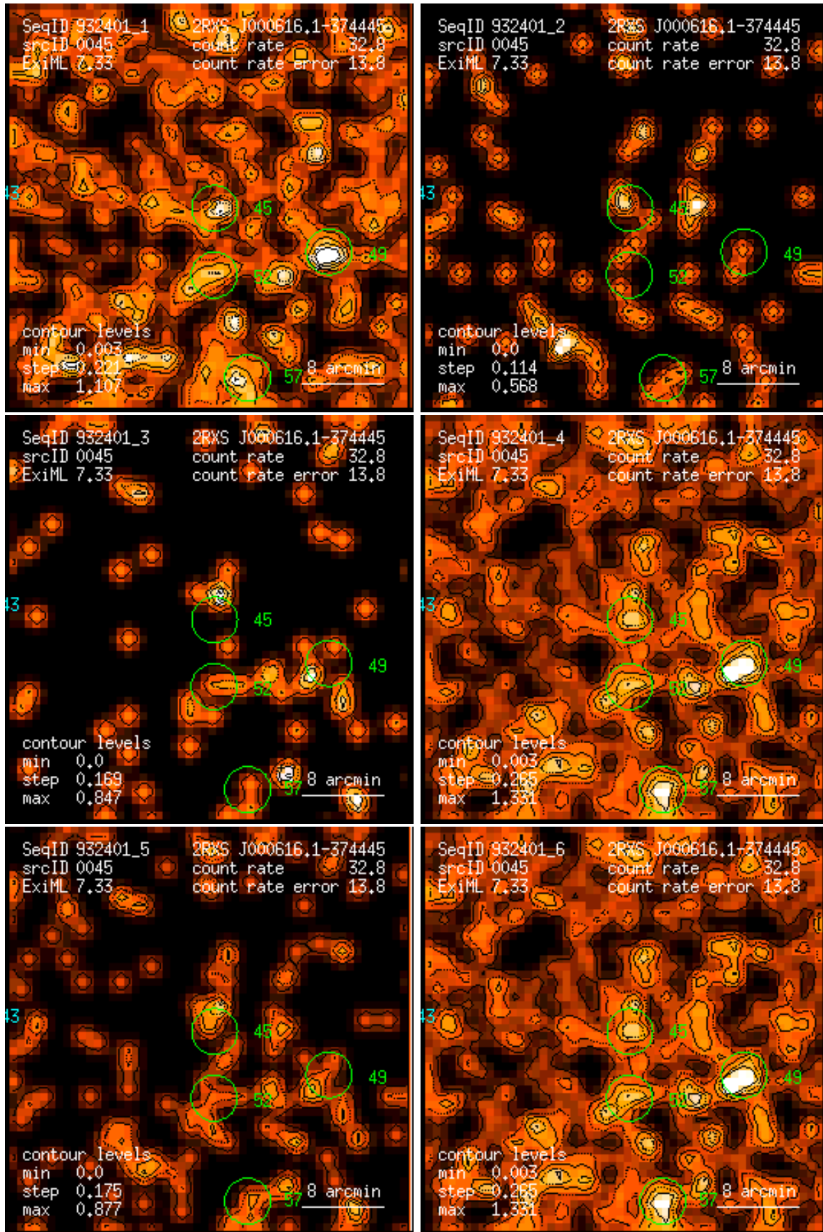
Figure 45: RASS 932401: detection 0045: band rate images, Gaussian filter: (1) PSPC channels 11 – 41, (2) 52 – 90, (3) 91 – 201, (4) 11 – 235, (5) 52 – 201, (6) 11 – 201. Broad band rates in counts/ks. Band rate contour levels in counts/ks/arcmin 2 .
