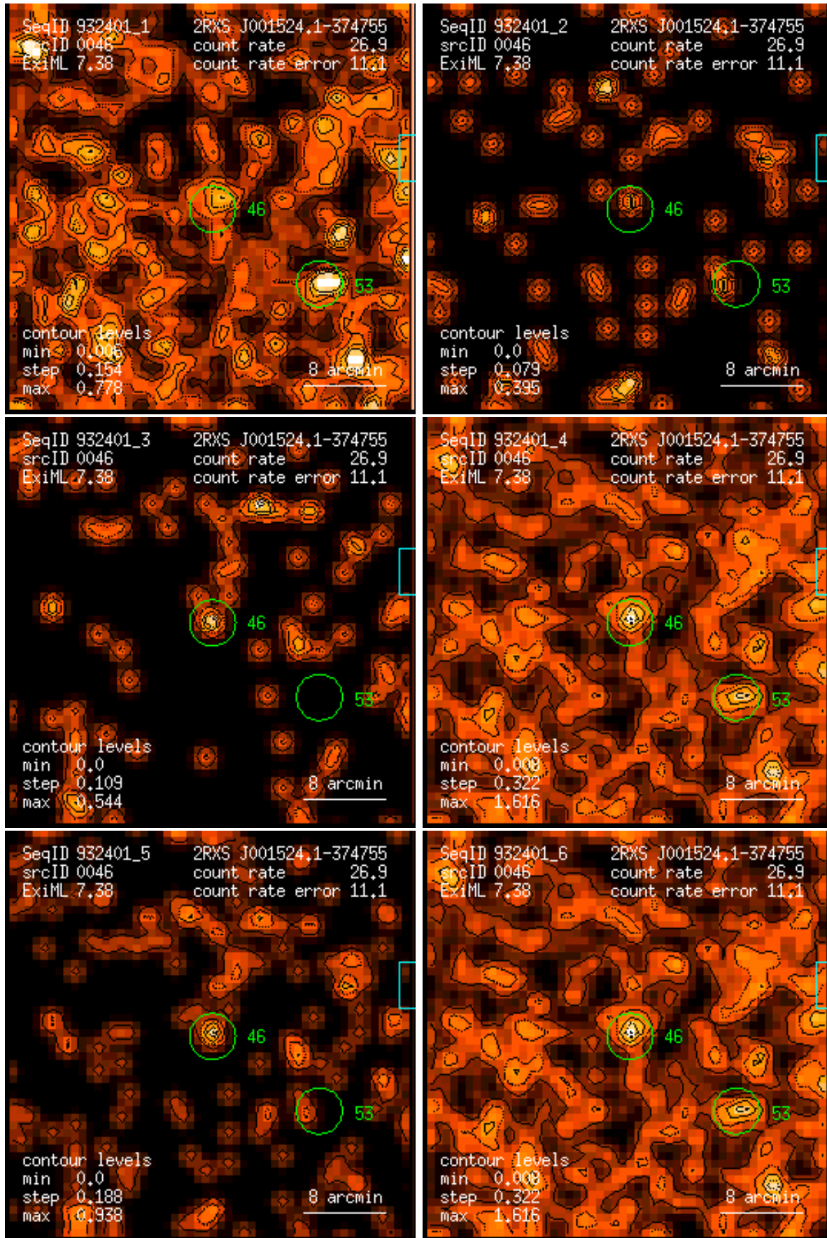
Figure 46: RASS 932401: detection 0046: band rate images, Gaussian filter: (1) PSPC channels 11 – 41, (2) 52 – 90, (3) 91 – 201, (4) 11 – 235, (5) 52 – 201, (6) 11 – 201. Broad band rates in counts/ks. Band rate contour levels in counts/ks/arcmin 2 .
