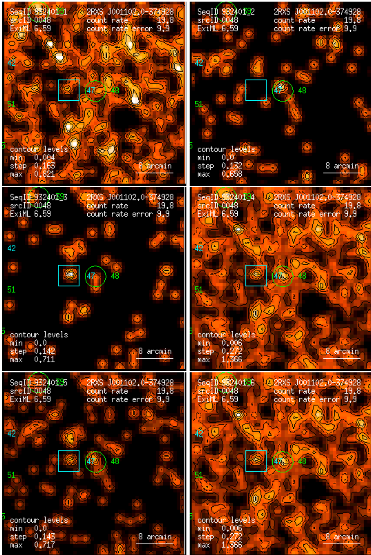
Figure 48: RASS 932401: detection 0048: band rate images, Gaussian filter: (1) PSPC channels 11 – 41, (2) 52 – 90, (3) 91 – 201, (4) 11 – 235, (5) 52 – 201, (6) 11 – 201. Broad band rates in counts/ks. Band rate contour levels in counts/ks/arcmin 2 .
