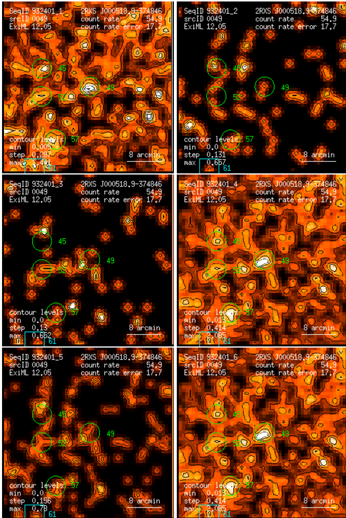
Figure 49: RASS 932401: detection 0049: band rate images, Gaussian filter: (1) PSPC channels 11 – 41, (2) 52 – 90, (3) 91 – 201, (4) 11 – 235, (5) 52 – 201, (6) 11 – 201. Broad band rates in counts/ks. Band rate contour levels in counts/ks/arcmin 2 .
