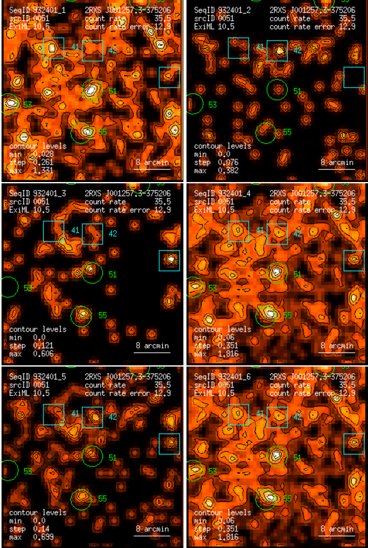
Figure 51: RASS 932401: detection 0051: band rate images, Gaussian filter: (1) PSPC channels 11 – 41, (2) 52 – 90, (3) 91 – 201, (4) 11 – 235, (5) 52 – 201, (6) 11 – 201. Broad band rates in counts/ks. Band rate contour levels in counts/ks/arcmin 2 .
