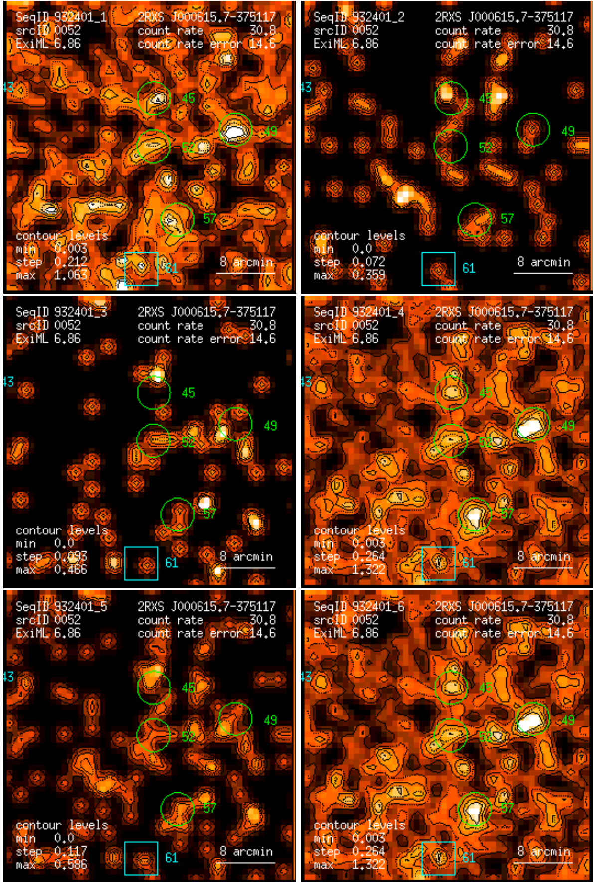
Figure 52: RASS 932401: detection 0052: band rate images, Gaussian filter: (1) PSPC channels 11 – 41, (2) 52 – 90, (3) 91 – 201, (4) 11 – 235, (5) 52 – 201, (6) 11 – 201. Broad band rates in counts/ks. Band rate contour levels in counts/ks/arcmin 2 .
