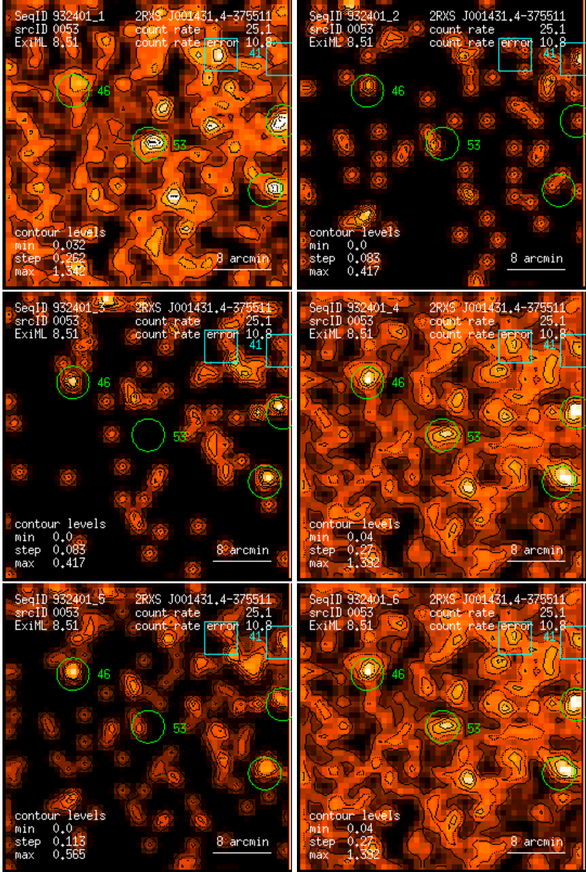
Figure 53: RASS 932401: detection 0053: band rate images, Gaussian filter: (1) PSPC channels 11 – 41, (2) 52 – 90, (3) 91 – 201, (4) 11 – 235, (5) 52 – 201, (6) 11 – 201. Broad band rates in counts/ks. Band rate contour levels in counts/ks/arcmin 2 .
