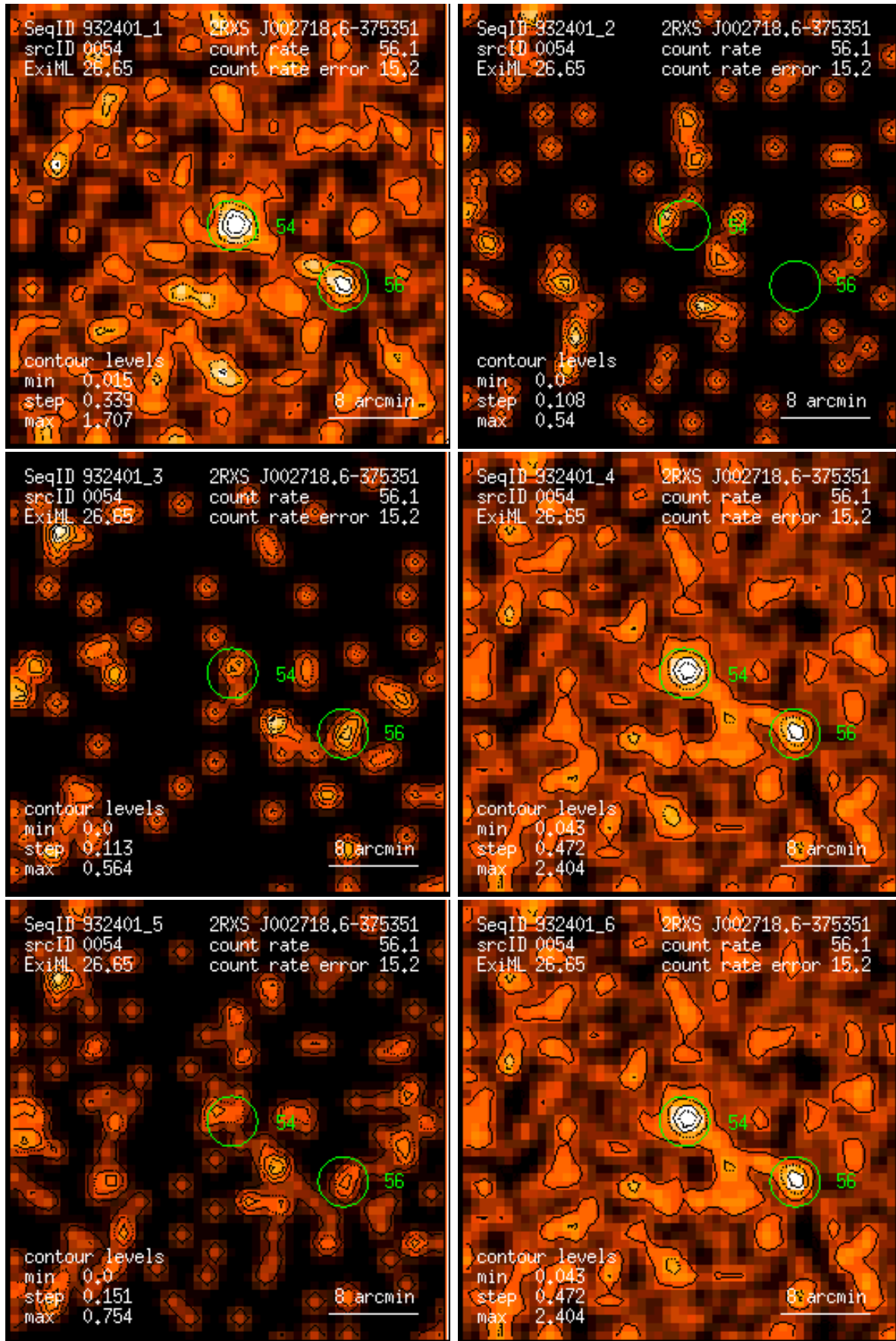
Figure 54: RASS 932401: detection 0054: band rate images, Gaussian filter: (1) PSPC channels 11 – 41, (2) 52 – 90, (3) 91 – 201, (4) 11 – 235, (5) 52 – 201, (6) 11 – 201. Broad band rates in counts/ks. Band rate contour levels in counts/ks/arcmin 2 .
