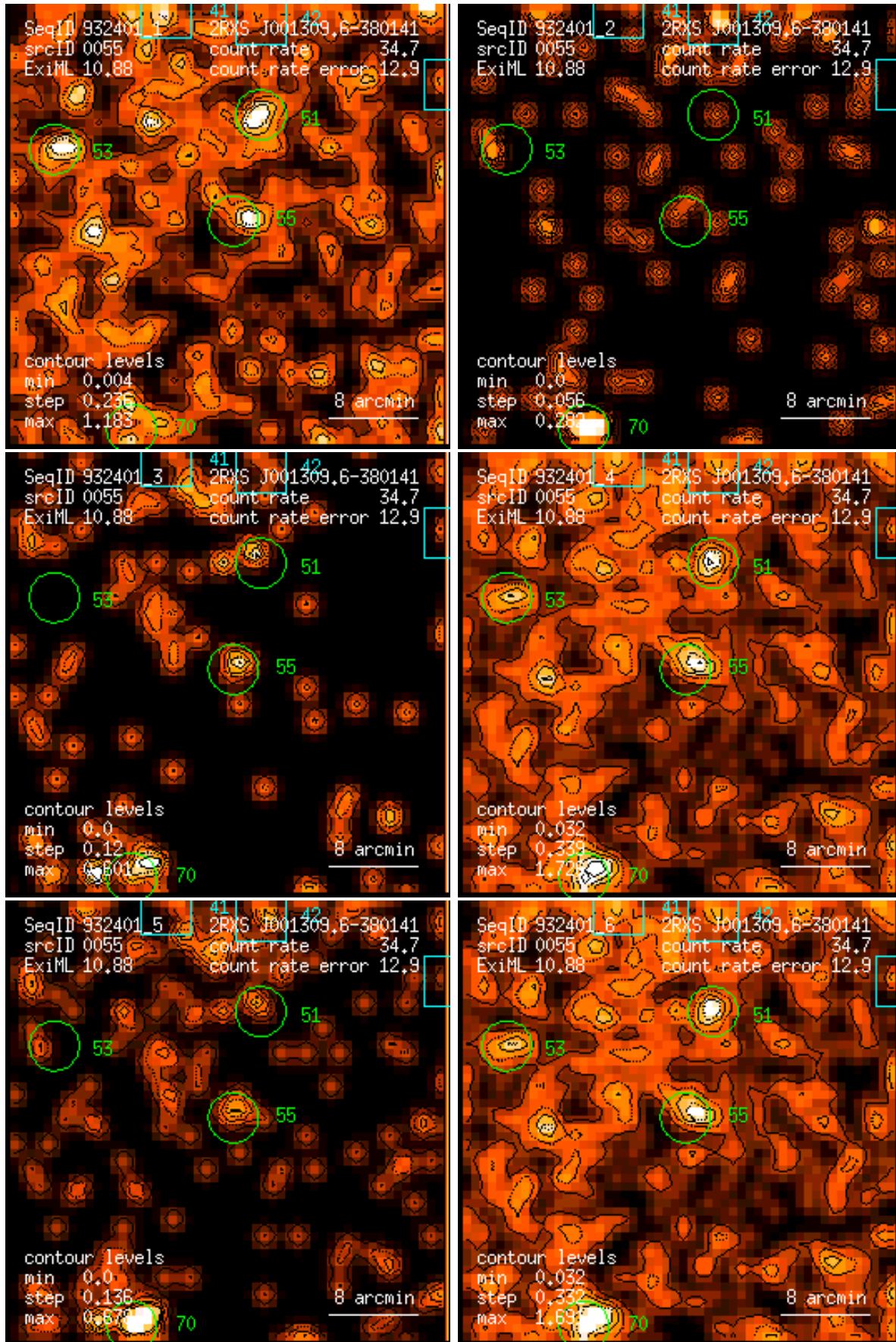
Figure 55: RASS 932401: detection 0055: band rate images, Gaussian filter: (1) PSPC channels 11 – 41, (2) 52 – 90, (3) 91 – 201, (4) 11 – 235, (5) 52 – 201, (6) 11 – 201. Broad band rates in counts/ks. Band rate contour levels in counts/ks/arcmin 2 .
