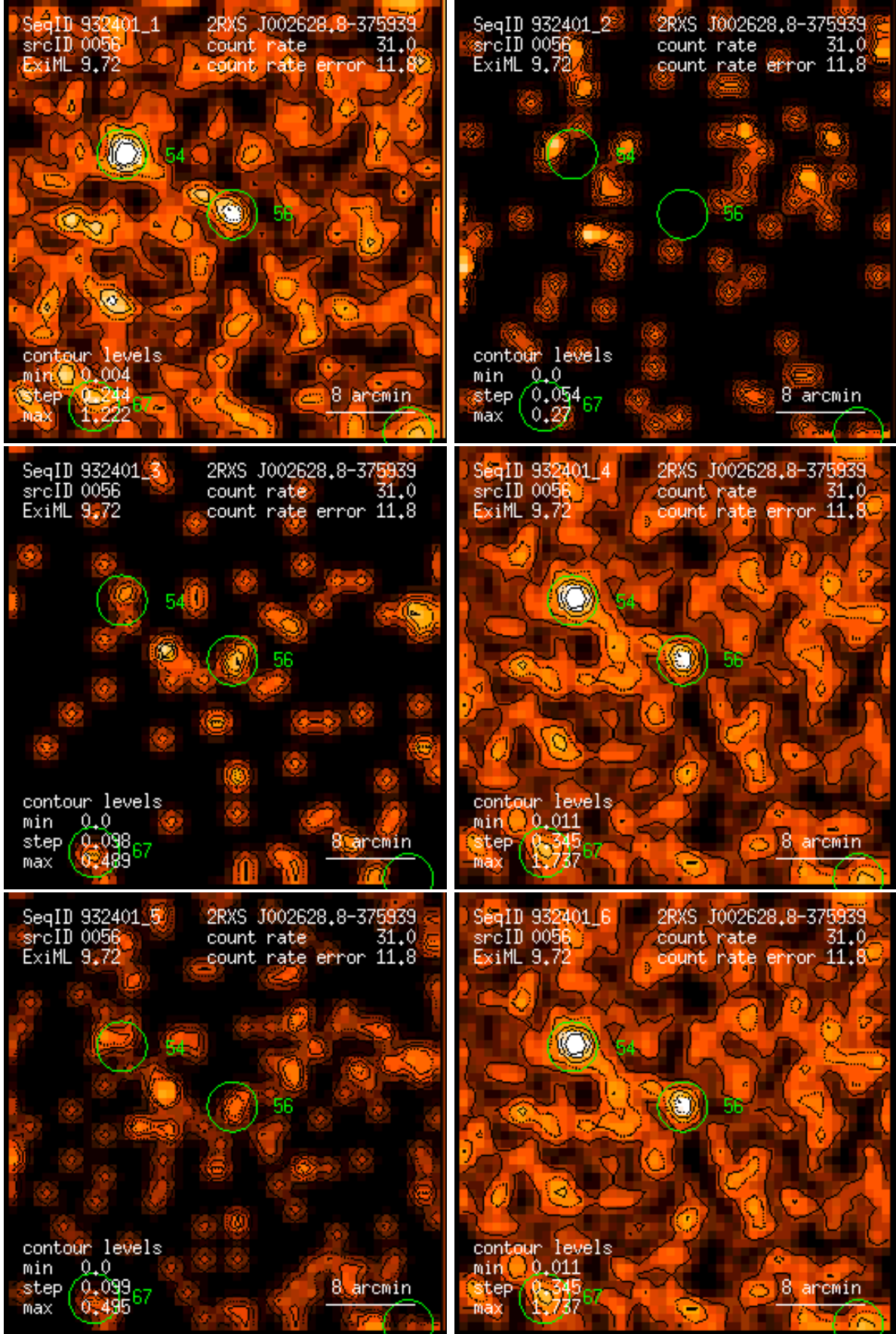
Figure 56: RASS 932401: detection 0056: band rate images, Gaussian filter: (1) PSPC channels 11 – 41, (2) 52 – 90, (3) 91 – 201, (4) 11 – 235, (5) 52 – 201, (6) 11 – 201. Broad band rates in counts/ks. Band rate contour levels in counts/ks/arcmin 2 .
