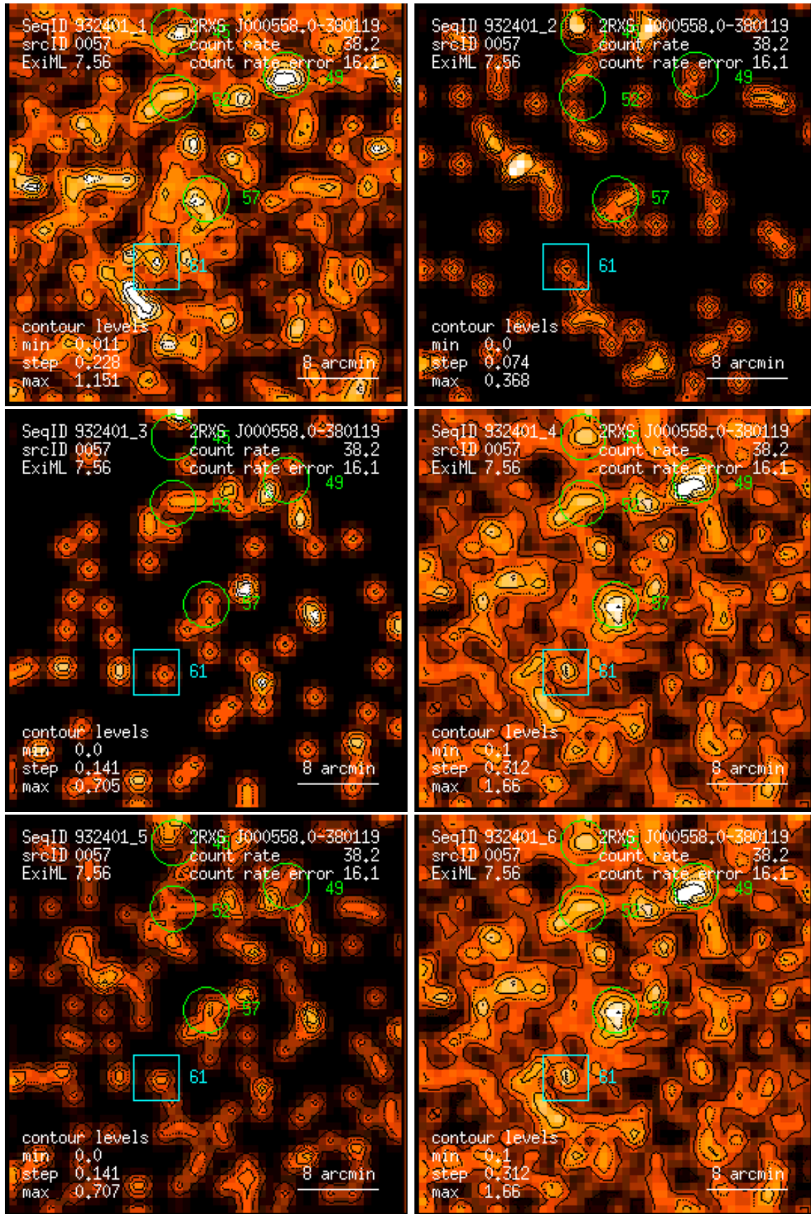
Figure 57: RASS 932401: detection 0057: band rate images, Gaussian filter: (1) PSPC channels 11 – 41, (2) 52 – 90, (3) 91 – 201, (4) 11 – 235, (5) 52 – 201, (6) 11 – 201. Broad band rates in counts/ks. Band rate contour levels in counts/ks/arcmin 2 .
