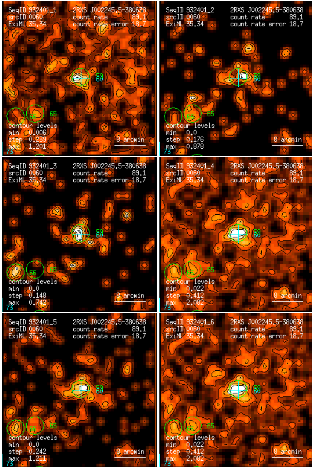
Figure 60: RASS 932401: detection 0060: band rate images, Gaussian filter: (1) PSPC channels 11 – 41, (2) 52 – 90, (3) 91 – 201, (4) 11 – 235, (5) 52 – 201, (6) 11 – 201. Broad band rates in counts/ks. Band rate contour levels in counts/ks/arcmin 2 .
