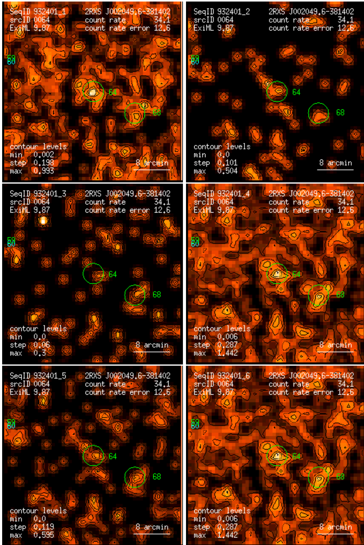
Figure 64: RASS 932401: detection 0064: band rate images, Gaussian filter: (1) PSPC channels 11 – 41, (2) 52 – 90, (3) 91 – 201, (4) 11 – 235, (5) 52 – 201, (6) 11 – 201. Broad band rates in counts/ks. Band rate contour levels in counts/ks/arcmin 2 .
