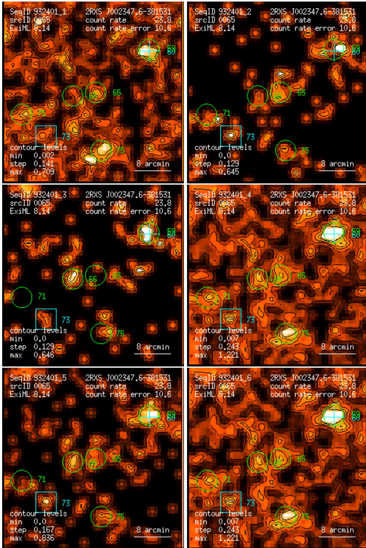
Figure 65: RASS 932401: detection 0065: band rate images, Gaussian filter: (1) PSPC channels 11 – 41, (2) 52 – 90, (3) 91 – 201, (4) 11 – 235, (5) 52 – 201, (6) 11 – 201. Broad band rates in counts/ks. Band rate contour levels in counts/ks/arcmin 2 .
