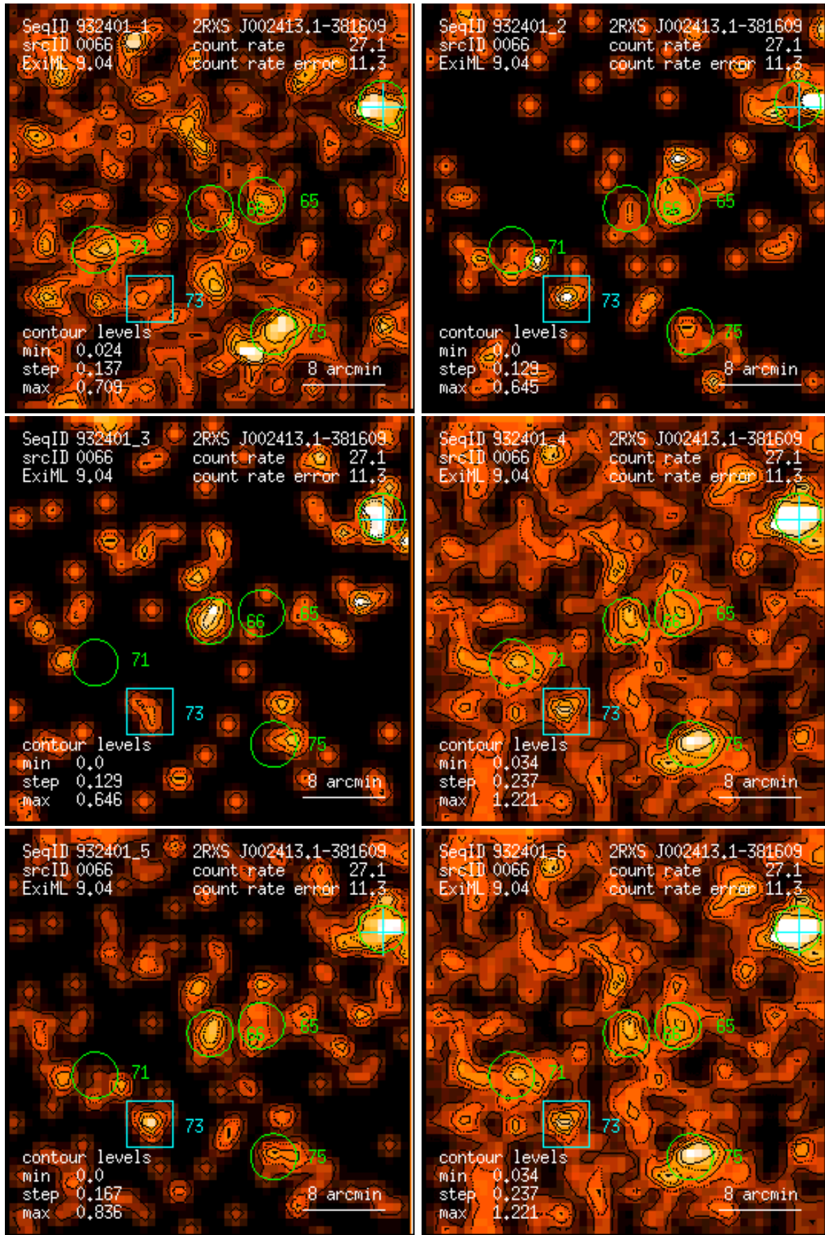
Figure 66: RASS 932401: detection 0066: band rate images, Gaussian filter: (1) PSPC channels 11 – 41, (2) 52 – 90, (3) 91 – 201, (4) 11 – 235, (5) 52 – 201, (6) 11 – 201. Broad band rates in counts/ks. Band rate contour levels in counts/ks/arcmin 2 .
