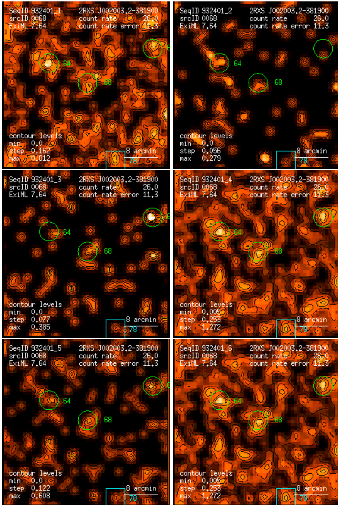
Figure 68: RASS 932401: detection 0068: band rate images, Gaussian filter: (1) PSPC channels 11 – 41, (2) 52 – 90, (3) 91 – 201, (4) 11 – 235, (5) 52 – 201, (6) 11 – 201. Broad band rates in counts/ks. Band rate contour levels in counts/ks/arcmin 2 .
