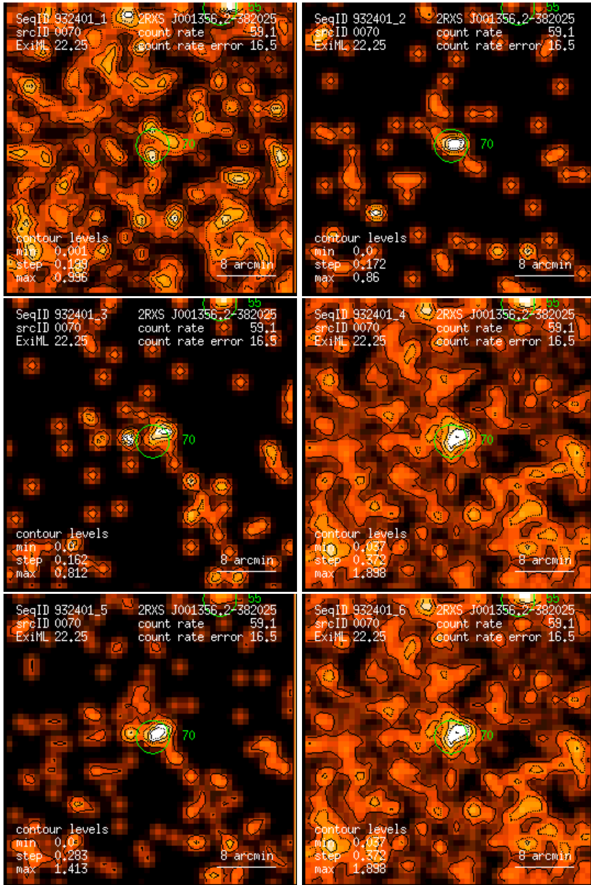
Figure 70: RASS 932401: detection 0070: band rate images, Gaussian filter: (1) PSPC channels 11 – 41, (2) 52 – 90, (3) 91 – 201, (4) 11 – 235, (5) 52 – 201, (6) 11 – 201. Broad band rates in counts/ks. Band rate contour levels in counts/ks/arcmin 2 .
