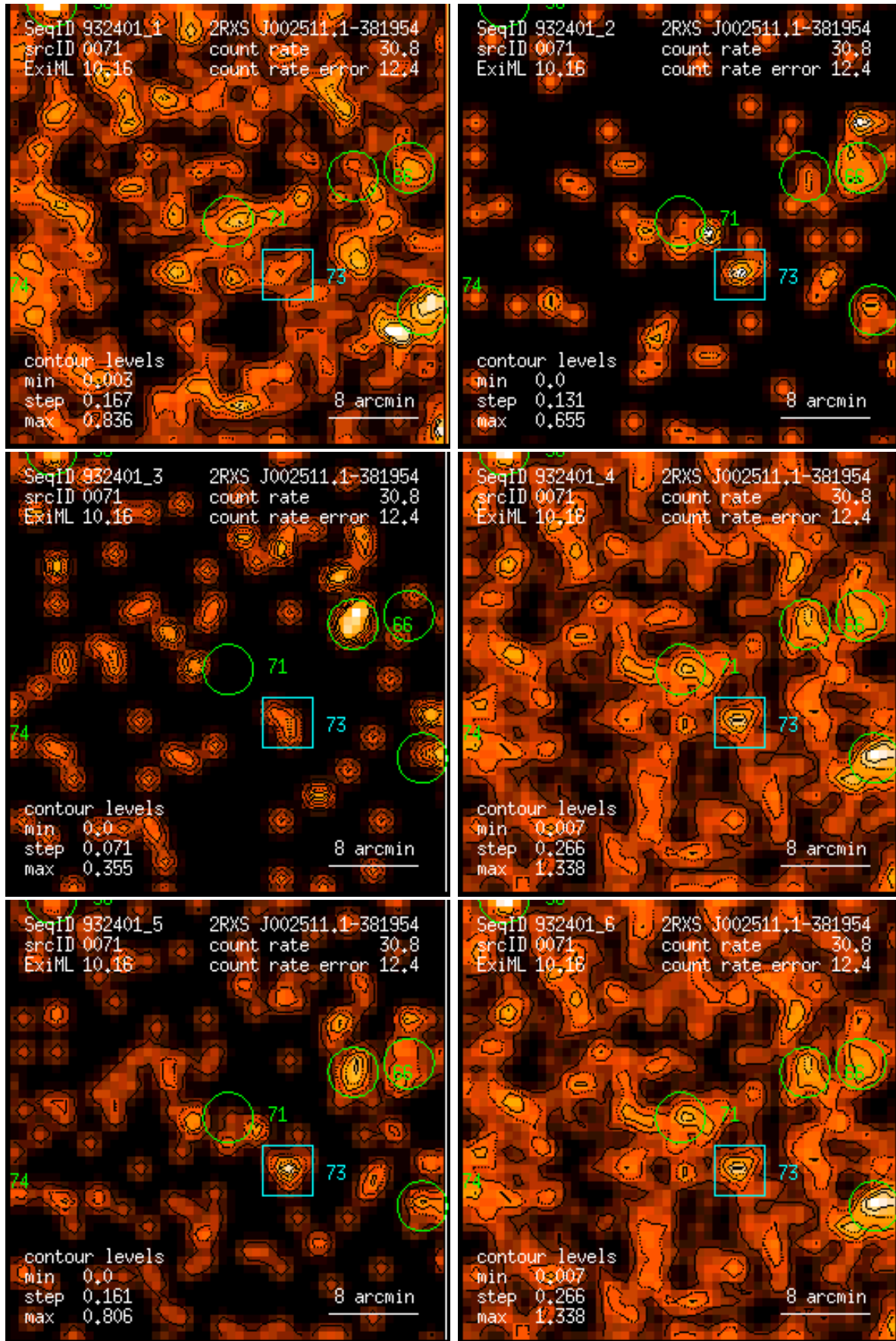
Figure 71: RASS 932401: detection 0071: band rate images, Gaussian filter: (1) PSPC channels 11 – 41, (2) 52 – 90, (3) 91 – 201, (4) 11 – 235, (5) 52 – 201, (6) 11 – 201. Broad band rates in counts/ks. Band rate contour levels in counts/ks/arcmin 2 .
