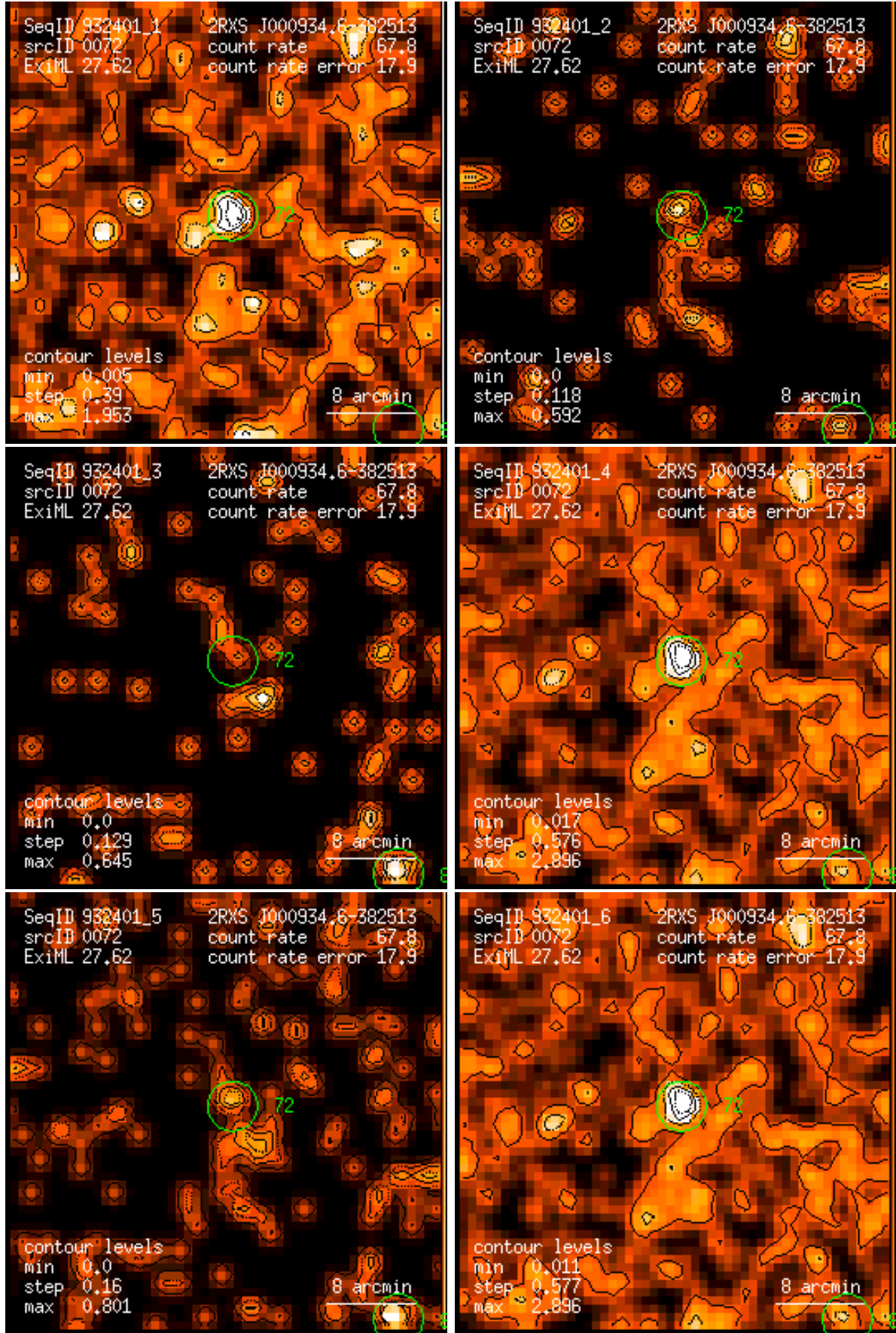
Figure 72: RASS 932401: detection 0072: band rate images, Gaussian filter: (1) PSPC channels 11 – 41, (2) 52 – 90, (3) 91 – 201, (4) 11 – 235, (5) 52 – 201, (6) 11 – 201. Broad band rates in counts/ks. Band rate contour levels in counts/ks/arcmin 2 .
