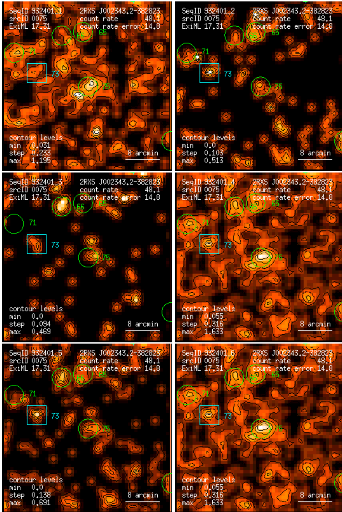
Figure 75: RASS 932401: detection 0075: band rate images, Gaussian filter: (1) PSPC channels 11 – 41, (2) 52 – 90, (3) 91 – 201, (4) 11 – 235, (5) 52 – 201, (6) 11 – 201. Broad band rates in counts/ks. Band rate contour levels in counts/ks/arcmin 2 .
