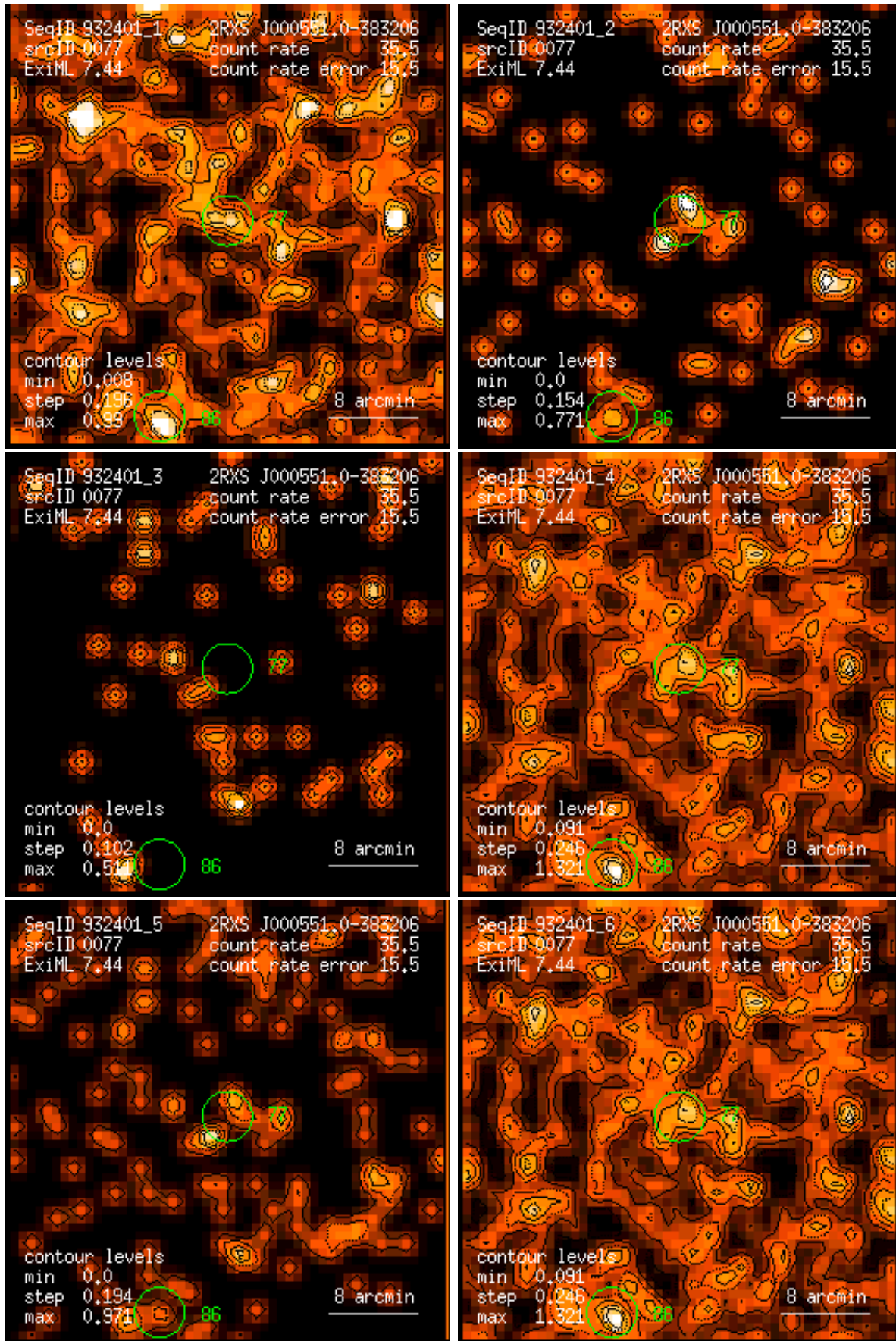
Figure 77: RASS 932401: detection 0077: band rate images, Gaussian filter: (1) PSPC channels 11 – 41, (2) 52 – 90, (3) 91 – 201, (4) 11 – 235, (5) 52 – 201, (6) 11 – 201. Broad band rates in counts/ks. Band rate contour levels in counts/ks/arcmin 2 .
