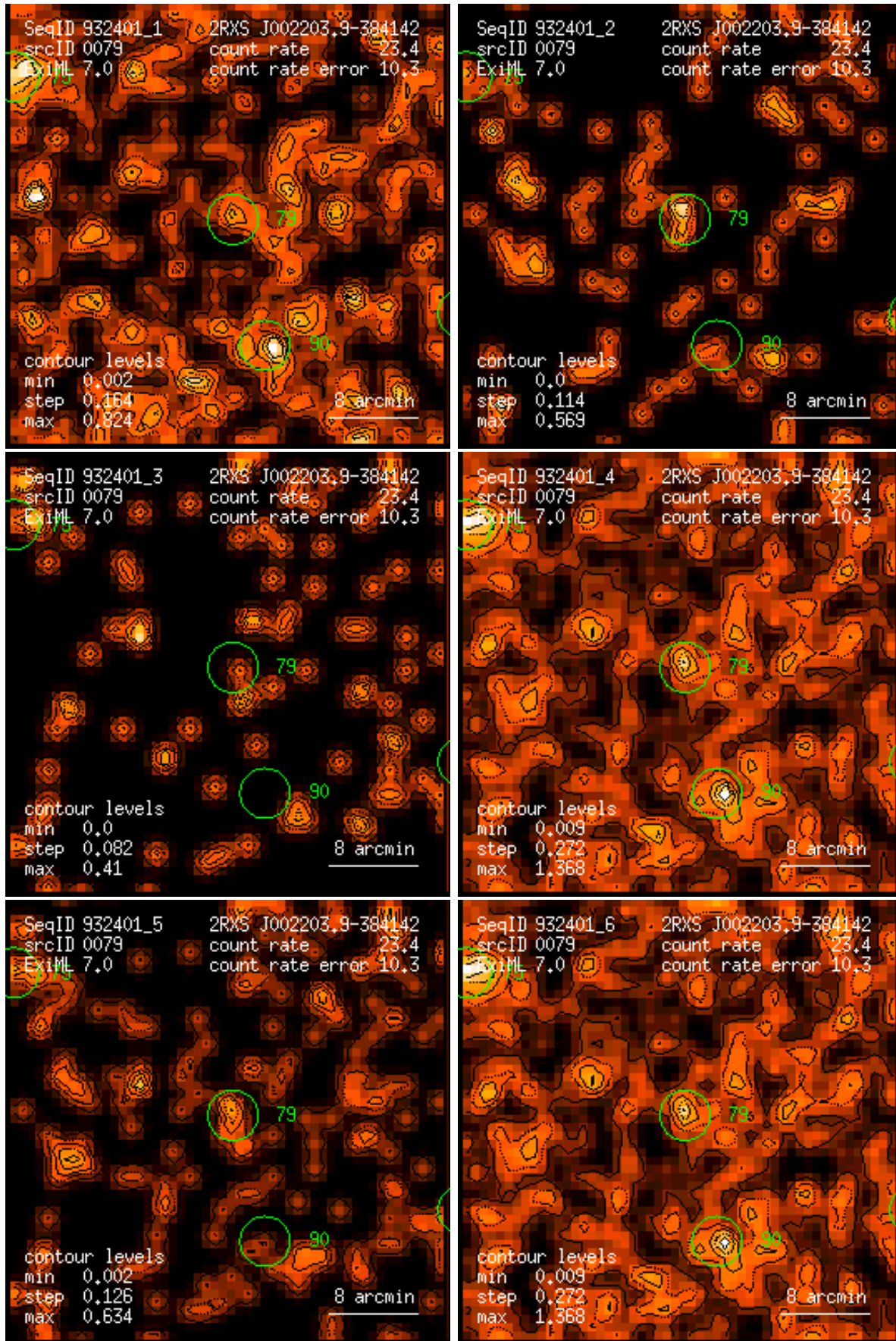
Figure 79: RASS 932401: detection 0079: band rate images, Gaussian filter: (1) PSPC channels 11 – 41, (2) 52 – 90, (3) 91 – 201, (4) 11 – 235, (5) 52 – 201, (6) 11 – 201. Broad band rates in counts/ks. Band rate contour levels in counts/ks/arcmin 2 .
