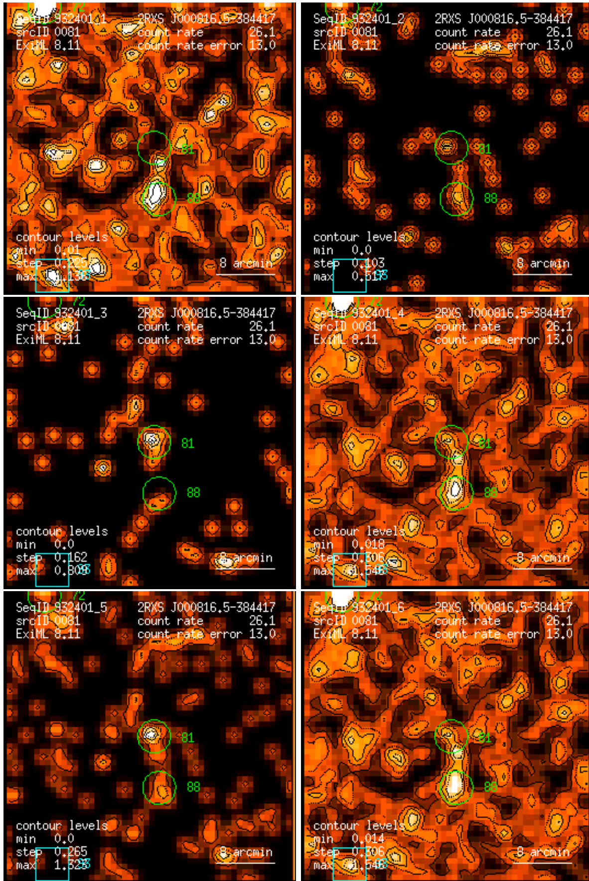
Figure 81: RASS 932401: detection 0081: band rate images, Gaussian filter: (1) PSPC channels 11 – 41, (2) 52 – 90, (3) 91 – 201, (4) 11 – 235, (5) 52 – 201, (6) 11 – 201. Broad band rates in counts/ks. Band rate contour levels in counts/ks/arcmin 2 .
