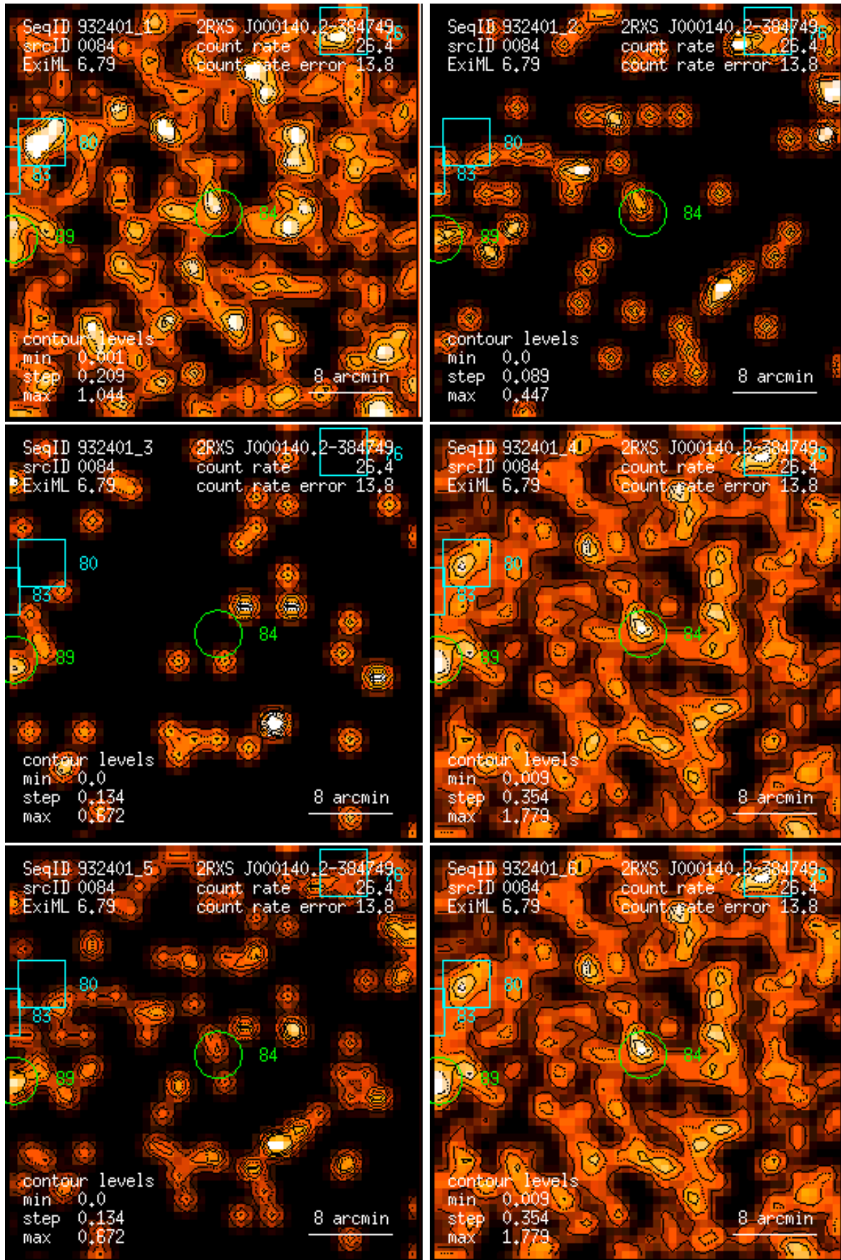
Figure 84: RASS 932401: detection 0084: band rate images, Gaussian filter: (1) PSPC channels 11 – 41, (2) 52 – 90, (3) 91 – 201, (4) 11 – 235, (5) 52 – 201, (6) 11 – 201. Broad band rates in counts/ks. Band rate contour levels in counts/ks/arcmin 2 .
