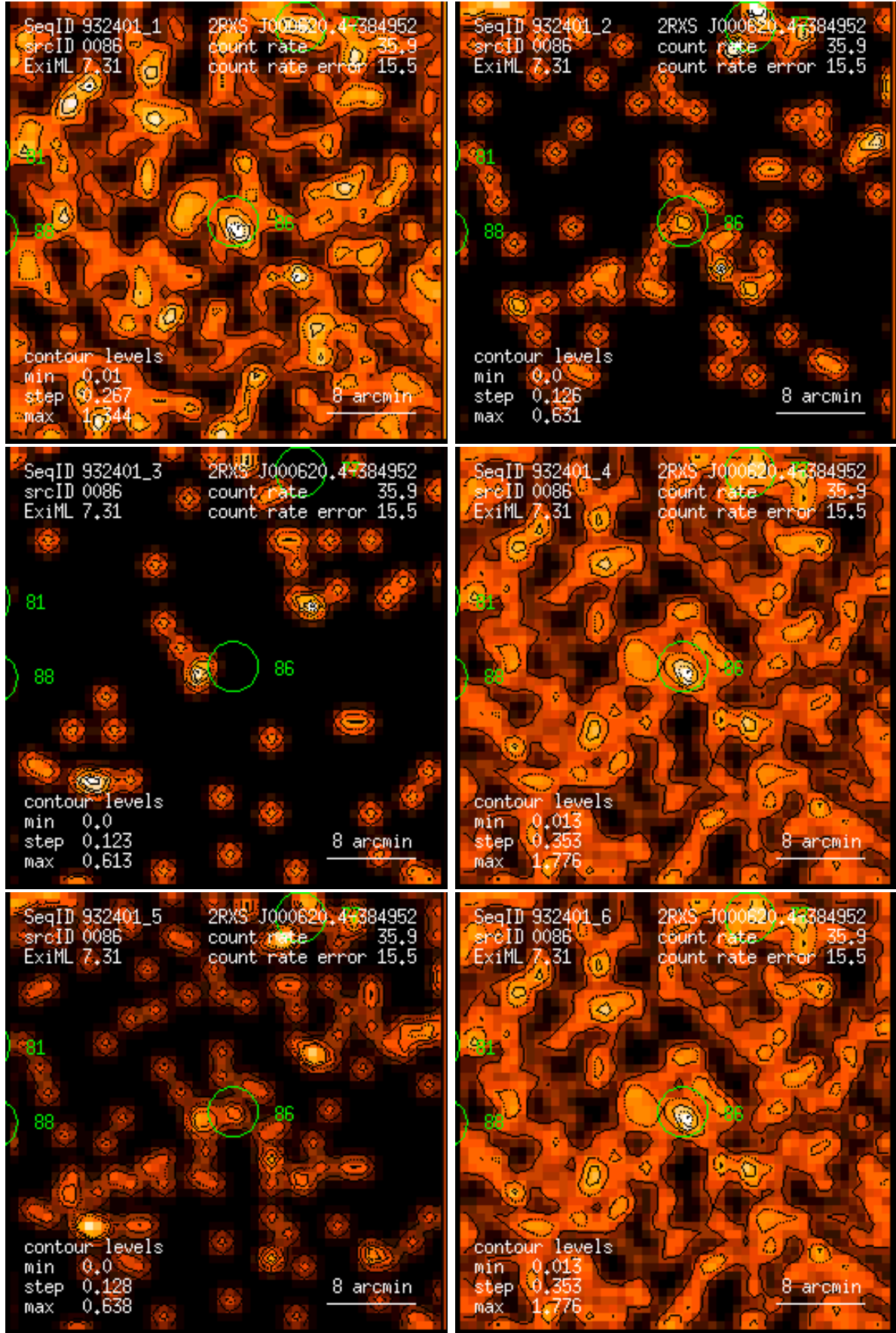
Figure 86: RASS 932401: detection 0086: band rate images, Gaussian filter: (1) PSPC channels 11 – 41, (2) 52 – 90, (3) 91 – 201, (4) 11 – 235, (5) 52 – 201, (6) 11 – 201. Broad band rates in counts/ks. Band rate contour levels in counts/ks/arcmin 2 .
