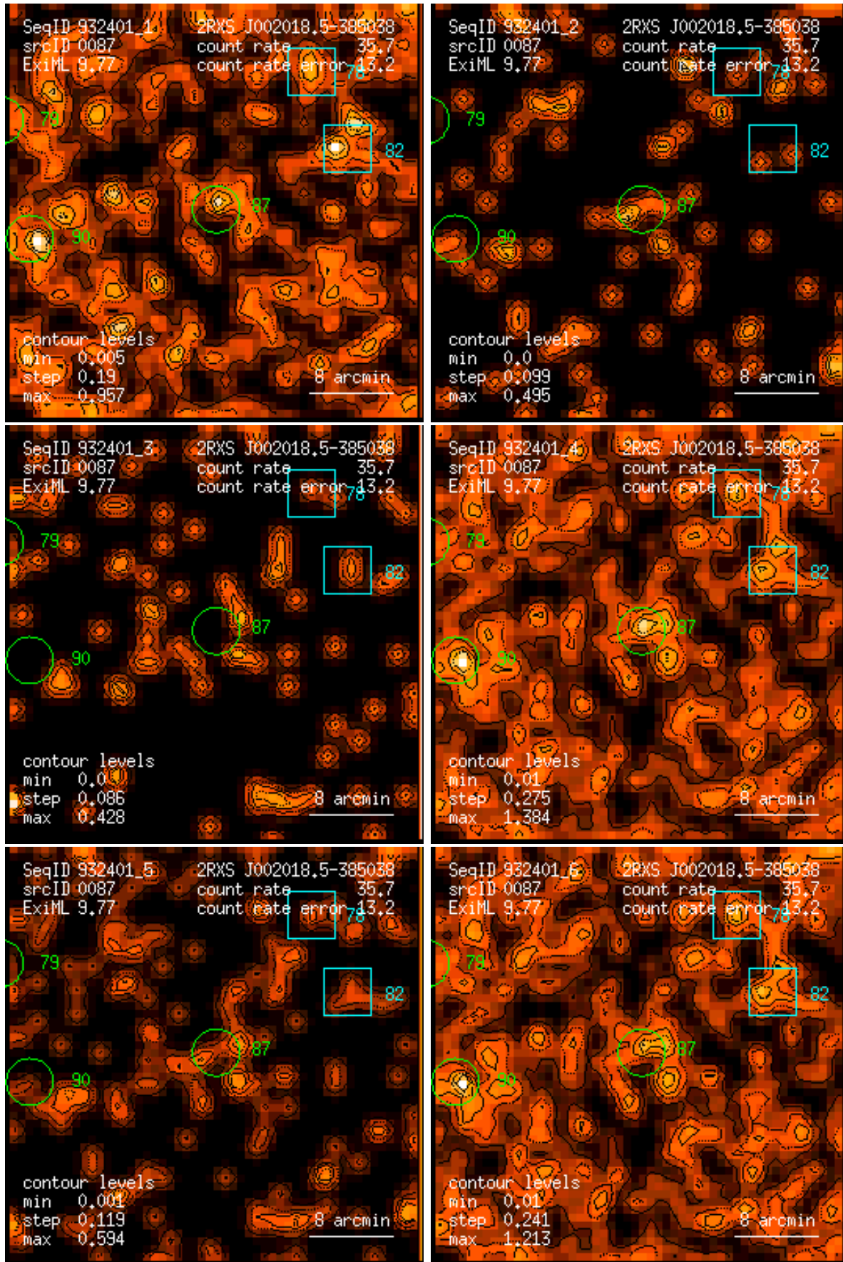
Figure 87: RASS 932401: detection 0087: band rate images, Gaussian filter: (1) PSPC channels 11 – 41, (2) 52 – 90, (3) 91 – 201, (4) 11 – 235, (5) 52 – 201, (6) 11 – 201. Broad band rates in counts/ks. Band rate contour levels in counts/ks/arcmin 2 .
