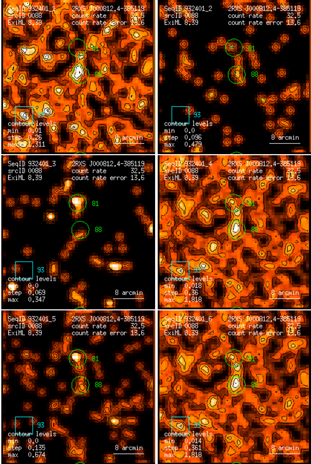
Figure 88: RASS 932401: detection 0088: band rate images, Gaussian filter: (1) PSPC channels 11 – 41, (2) 52 – 90, (3) 91 – 201, (4) 11 – 235, (5) 52 – 201, (6) 11 – 201. Broad band rates in counts/ks. Band rate contour levels in counts/ks/arcmin 2 .
