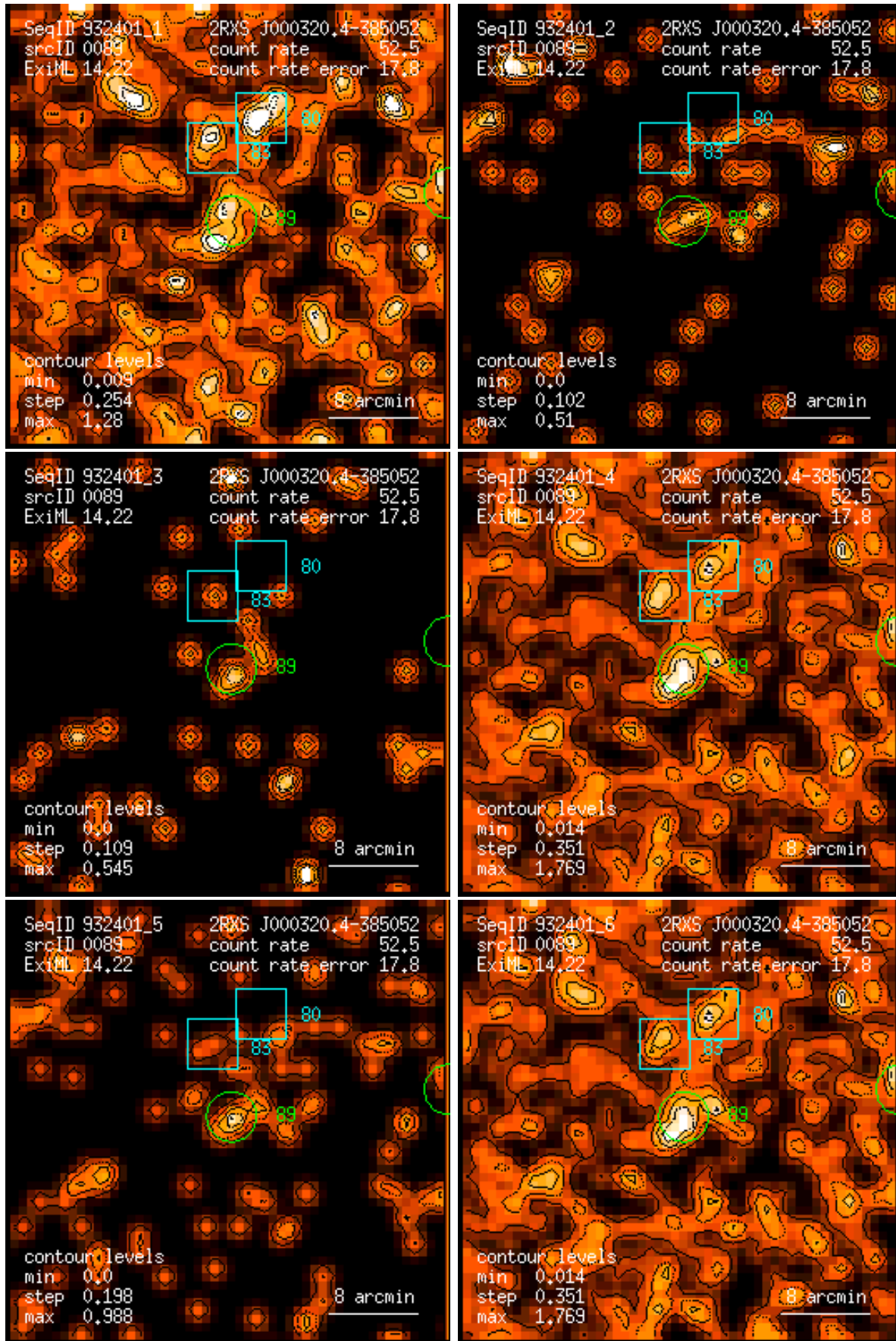
Figure 89: RASS 932401: detection 0089: band rate images, Gaussian filter: (1) PSPC channels 11 – 41, (2) 52 – 90, (3) 91 – 201, (4) 11 – 235, (5) 52 – 201, (6) 11 – 201. Broad band rates in counts/ks. Band rate contour levels in counts/ks/arcmin 2 .
