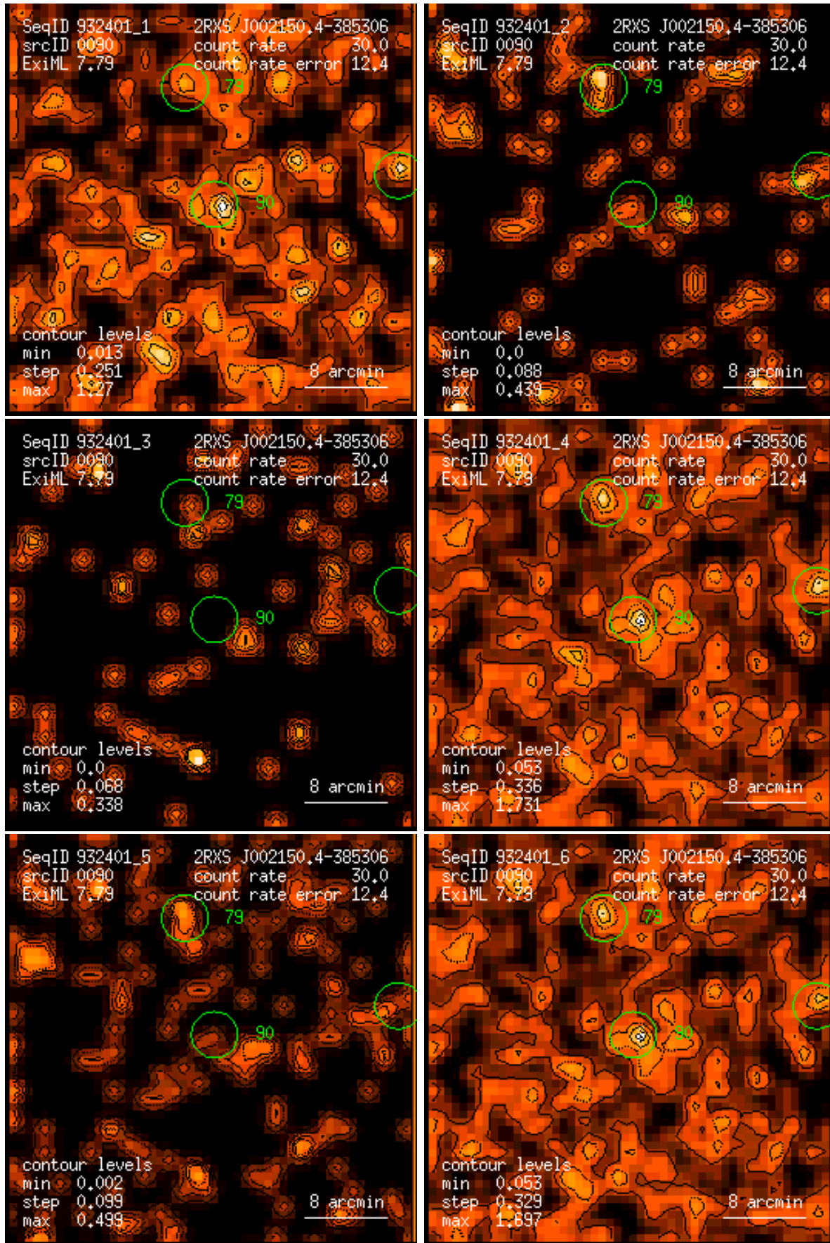
Figure 90: RASS 932401: detection 0090: band rate images, Gaussian filter: (1) PSPC channels 11 – 41, (2) 52 – 90, (3) 91 – 201, (4) 11 – 235, (5) 52 – 201, (6) 11 – 201. Broad band rates in counts/ks. Band rate contour levels in counts/ks/arcmin 2 .
