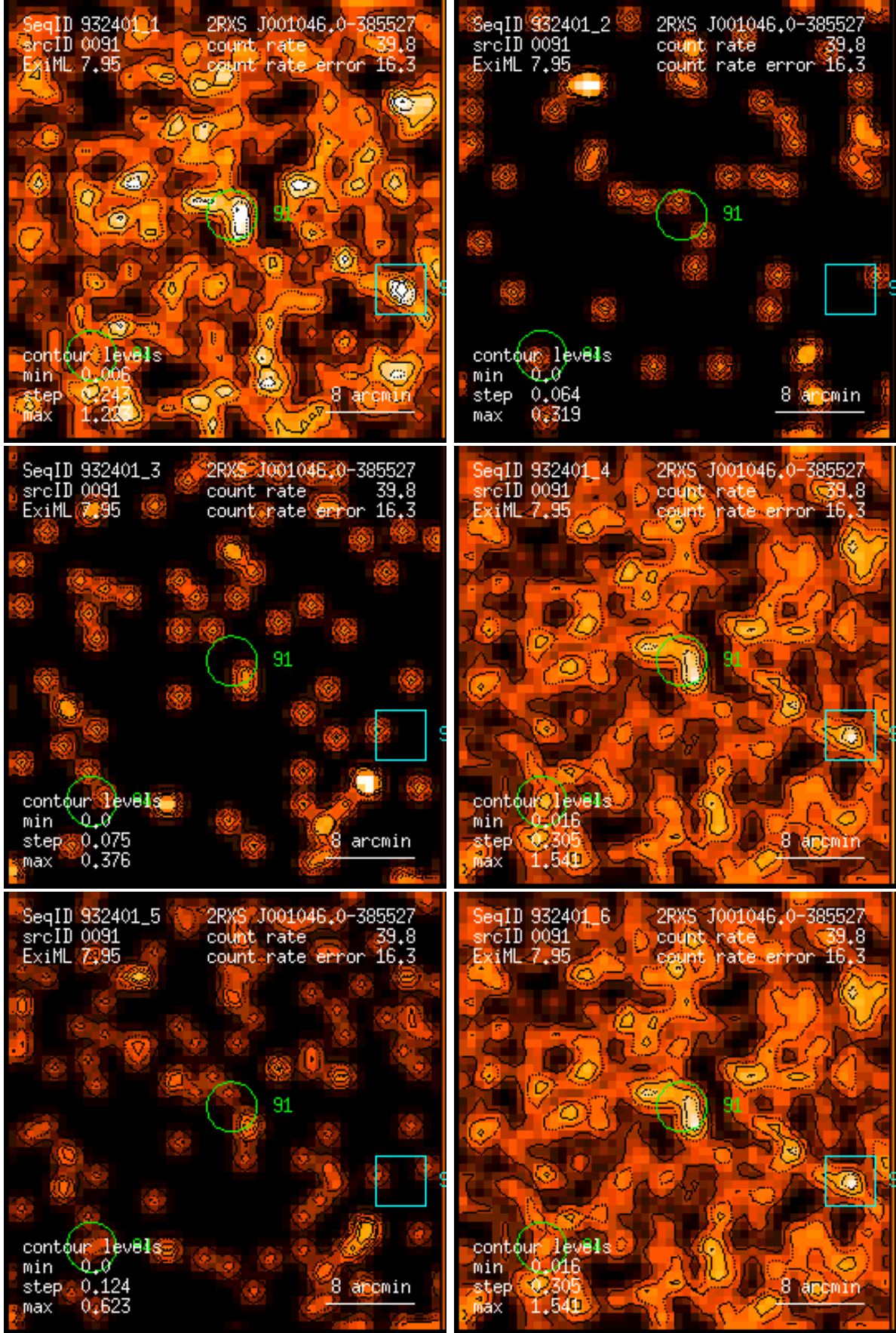
Figure 91: RASS 932401: detection 0091: band rate images, Gaussian filter: (1) PSPC channels 11 – 41, (2) 52 – 90, (3) 91 – 201, (4) 11 – 235, (5) 52 – 201, (6) 11 – 201. Broad band rates in counts/ks. Band rate contour levels in counts/ks/arcmin 2 .
