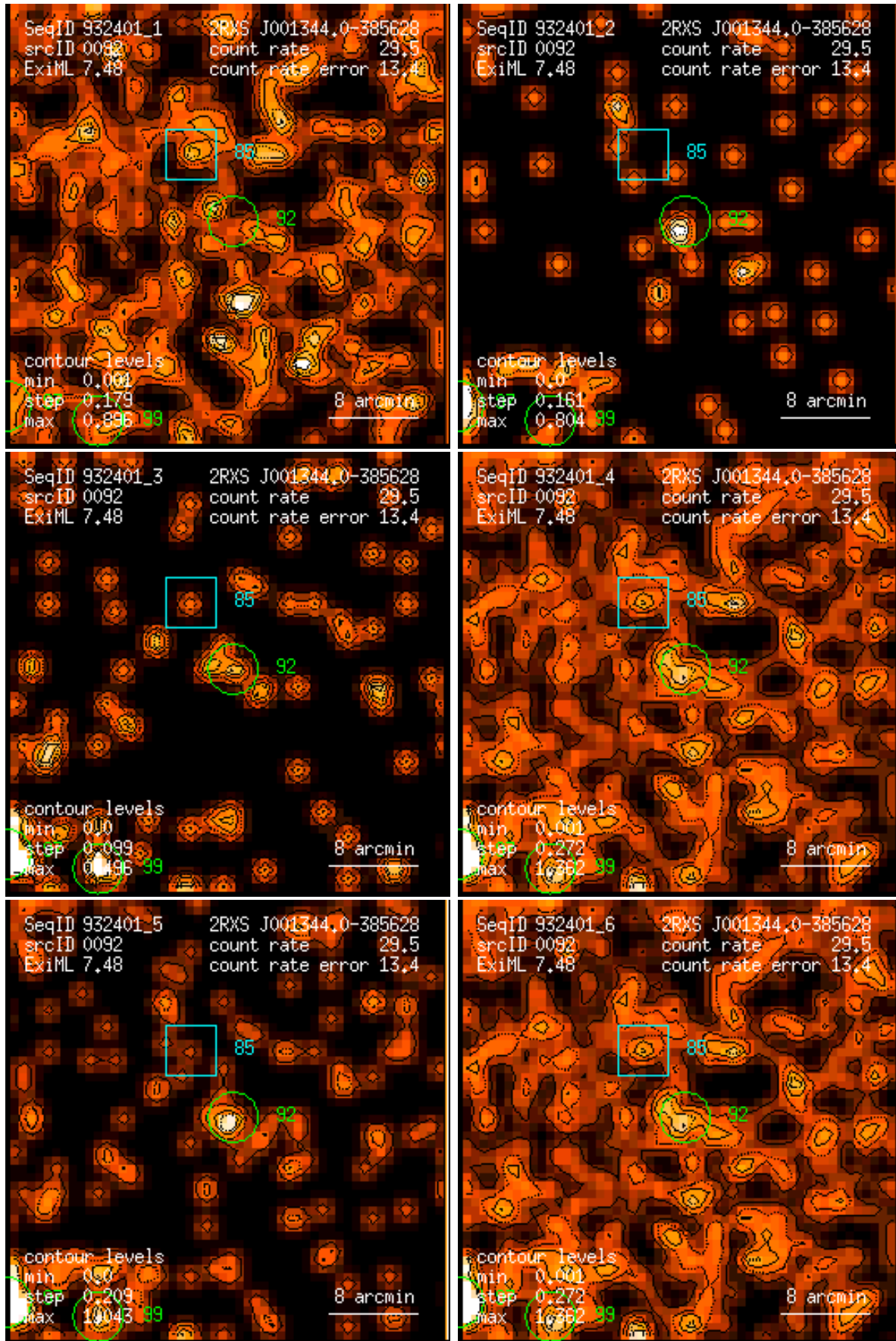
Figure 92: RASS 932401: detection 0092: band rate images, Gaussian filter: (1) PSPC channels 11 – 41, (2) 52 – 90, (3) 91 – 201, (4) 11 – 235, (5) 52 – 201, (6) 11 – 201. Broad band rates in counts/ks. Band rate contour levels in counts/ks/arcmin 2 .
