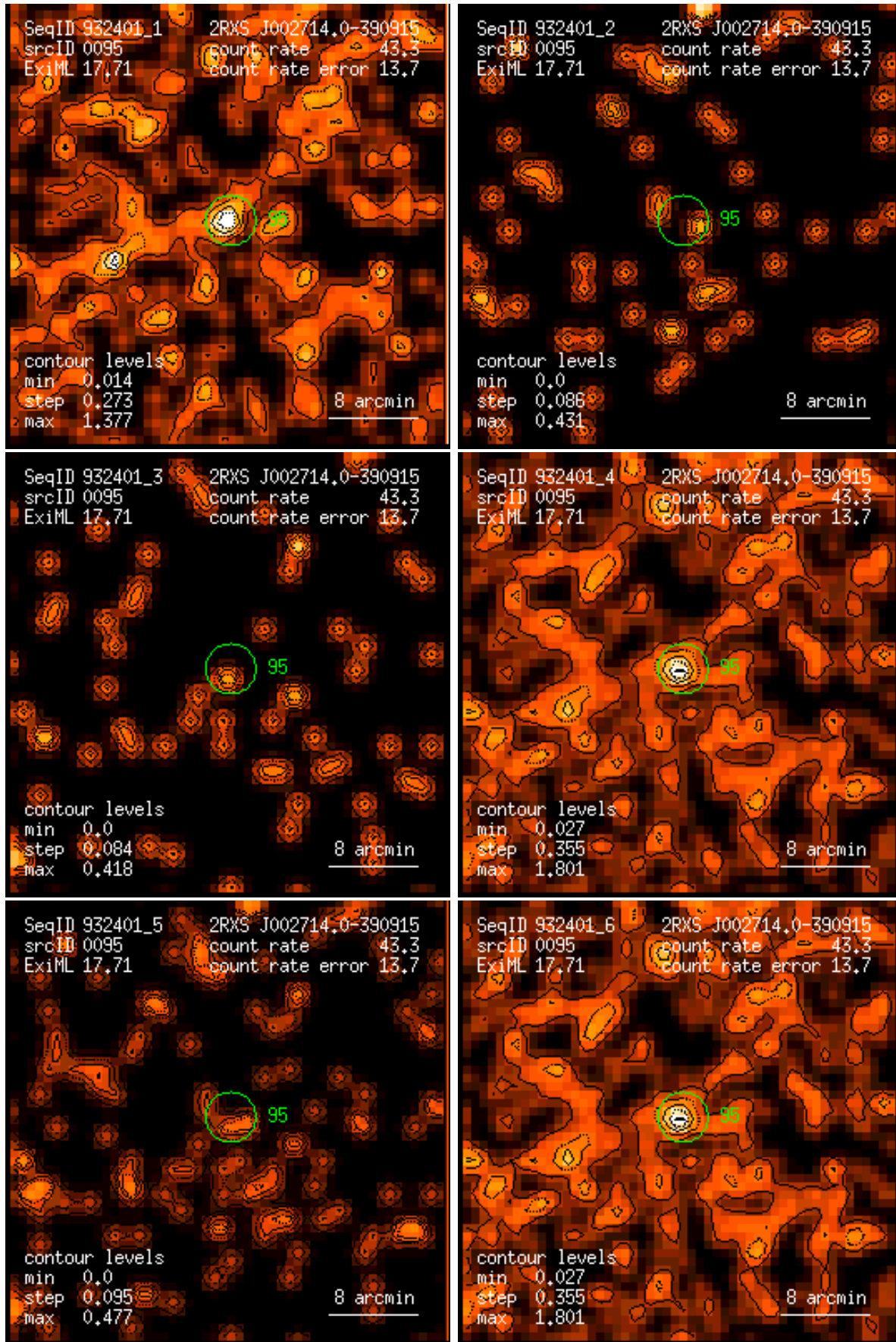
Figure 95: RASS 932401: detection 0095: band rate images, Gaussian filter: (1) PSPC channels 11 – 41, (2) 52 – 90, (3) 91 – 201, (4) 11 – 235, (5) 52 – 201, (6) 11 – 201. Broad band rates in counts/ks. Band rate contour levels in counts/ks/arcmin 2 .
