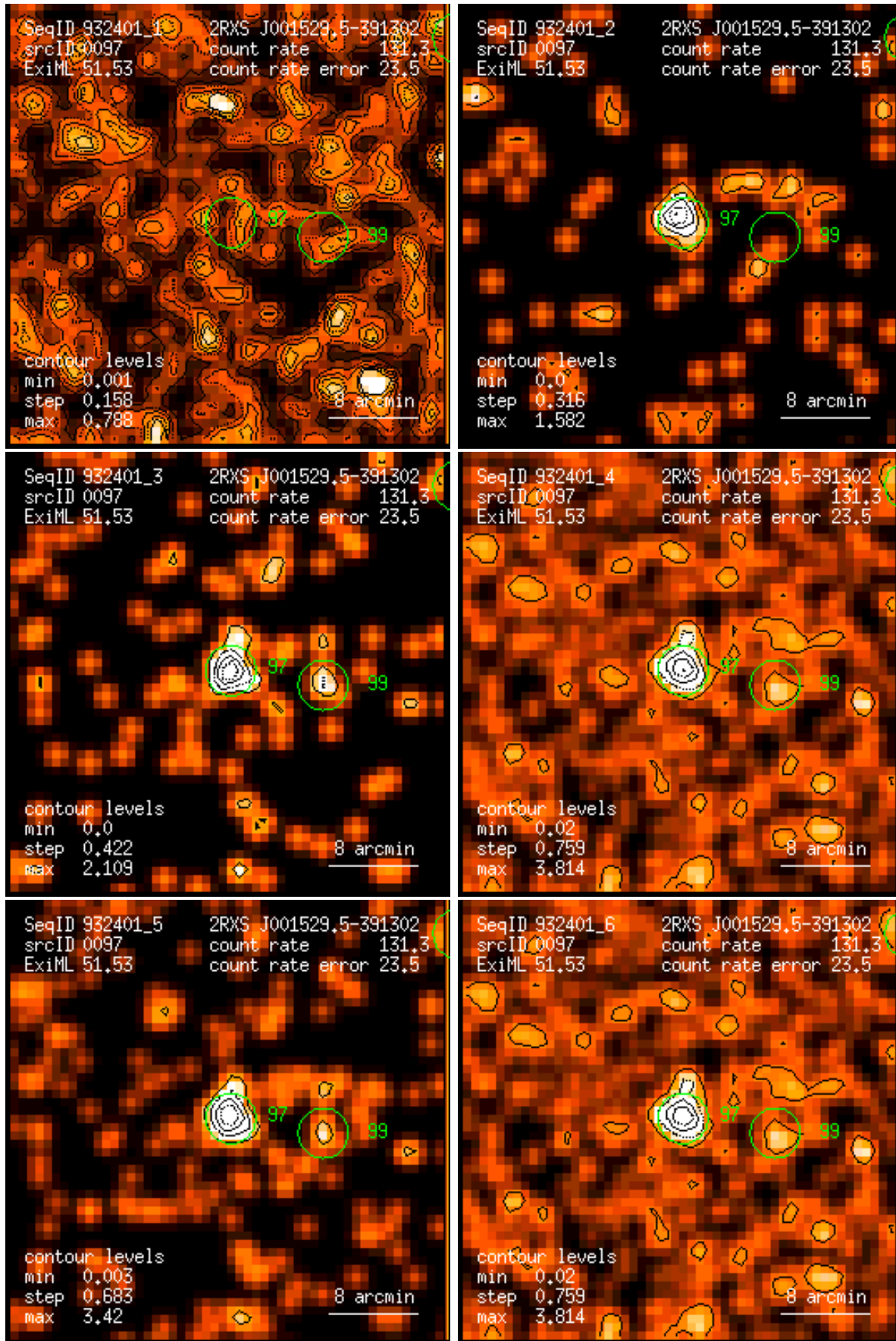
Figure 97: RASS 932401: detection 0097: band rate images, Gaussian filter: (1) PSPC channels 11 – 41, (2) 52 – 90, (3) 91 – 201, (4) 11 – 235, (5) 52 – 201, (6) 11 – 201. Broad band rates in counts/ks. Band rate contour levels in counts/ks/arcmin 2 .
