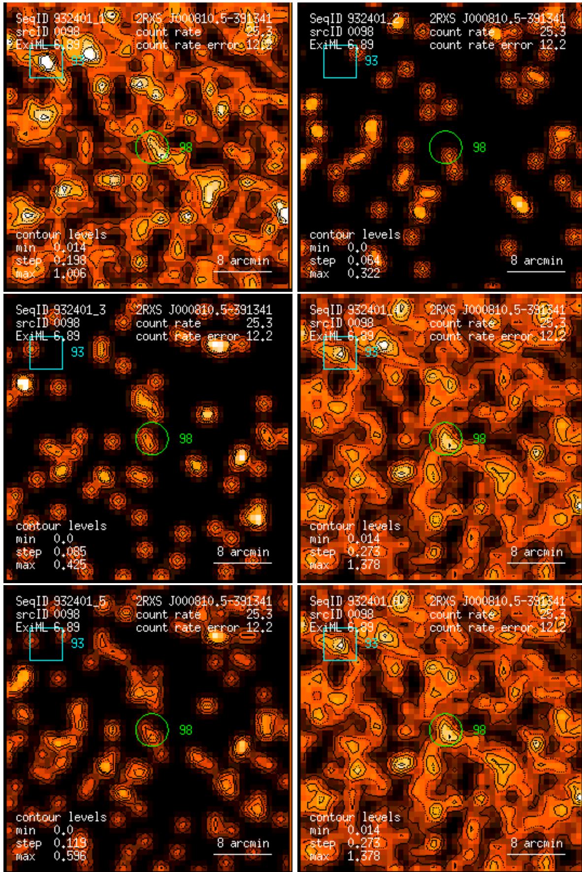
Figure 98: RASS 932401: detection 0098: band rate images, Gaussian filter: (1) PSPC channels 11 – 41, (2) 52 – 90, (3) 91 – 201, (4) 11 – 235, (5) 52 – 201, (6) 11 – 201. Broad band rates in counts/ks. Band rate contour levels in counts/ks/arcmin 2 .
