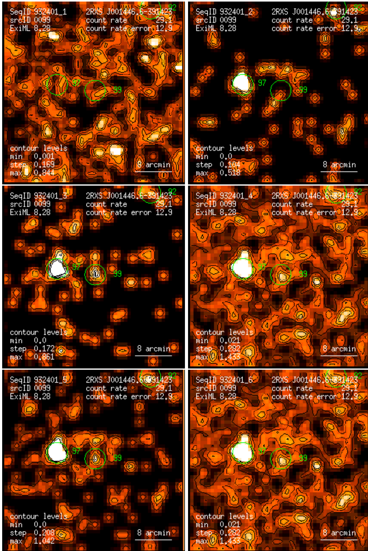
Figure 99: RASS 932401: detection 0099: band rate images, Gaussian filter: (1) PSPC channels 11 – 41, (2) 52 – 90, (3) 91 – 201, (4) 11 – 235, (5) 52 – 201, (6) 11 – 201. Broad band rates in counts/ks. Band rate contour levels in counts/ks/arcmin 2 .
