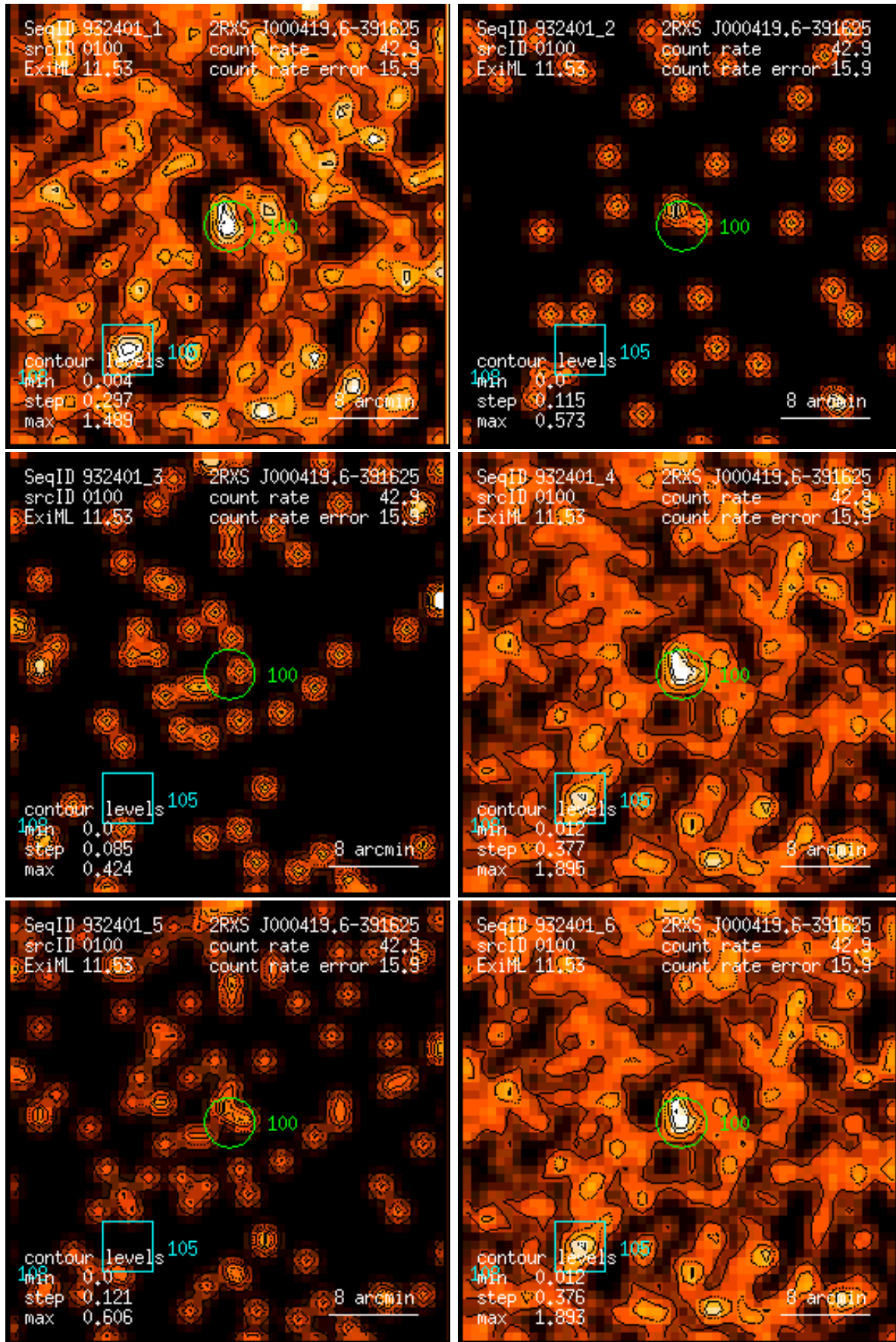
Figure 100: RASS 932401: detection 0100: band rate images, Gaussian filter: (1) PSPC channels 11 – 41, (2) 52 – 90, (3) 91 – 201, (4) 11 – 235, (5) 52 – 201, (6) 11 – 201. Broad band rates in counts/ks. Band rate contour levels in counts/ks/arcmin 2 .
