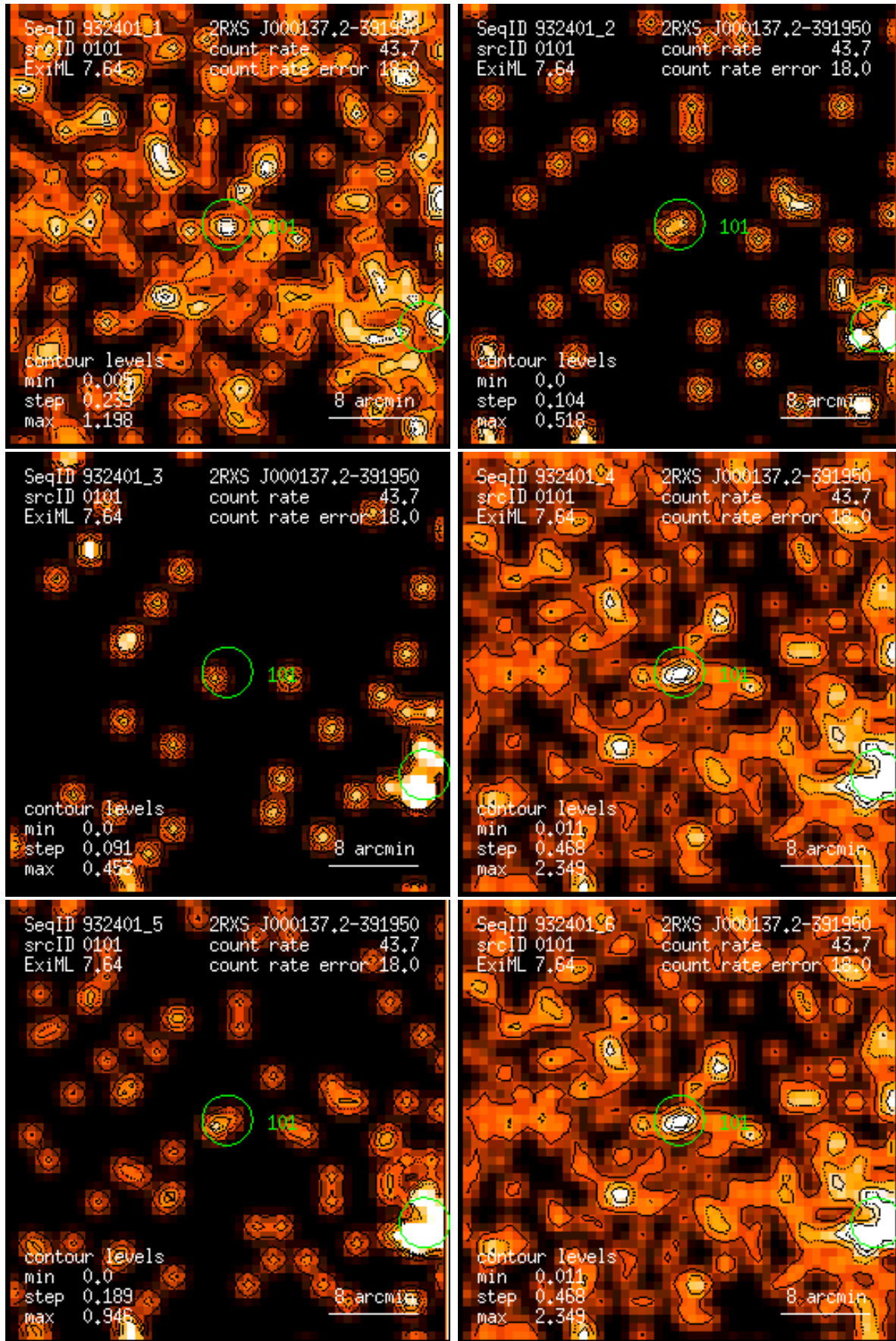
Figure 101: RASS 932401: detection 0101: band rate images, Gaussian filter: (1) PSPC channels 11 – 41, (2) 52 – 90, (3) 91 – 201, (4) 11 – 235, (5) 52 – 201, (6) 11 – 201. Broad band rates in counts/ks. Band rate contour levels in counts/ks/arcmin 2 .
