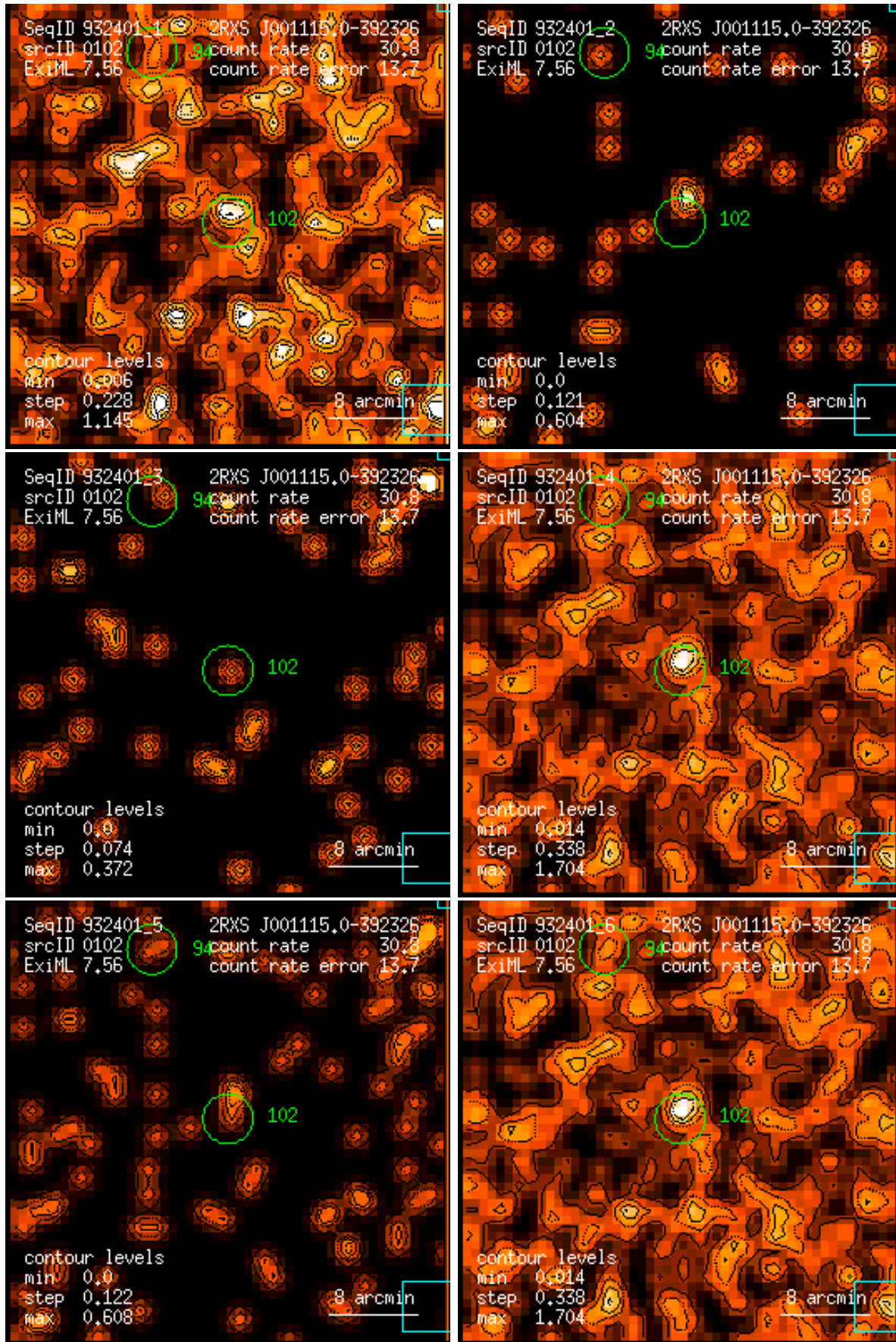
Figure 102: RASS 932401: detection 0102: band rate images, Gaussian filter: (1) PSPC channels 11 – 41, (2) 52 – 90, (3) 91 – 201, (4) 11 – 235, (5) 52 – 201, (6) 11 – 201. Broad band rates in counts/ks. Band rate contour levels in counts/ks/arcmin 2 .
