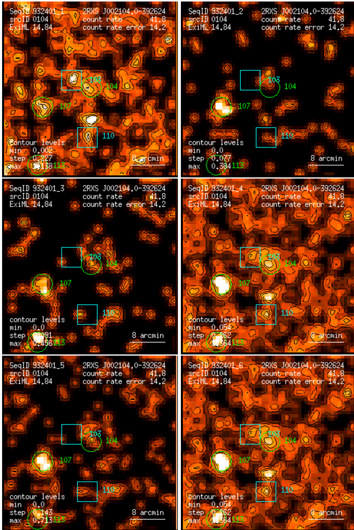
Figure 104: RASS 932401: detection 0104: band rate images, Gaussian filter: (1) PSPC channels 11 – 41, (2) 52 – 90, (3) 91 – 201, (4) 11 – 235, (5) 52 – 201, (6) 11 – 201. Broad band rates in counts/ks. Band rate contour levels in counts/ks/arcmin 2 .
