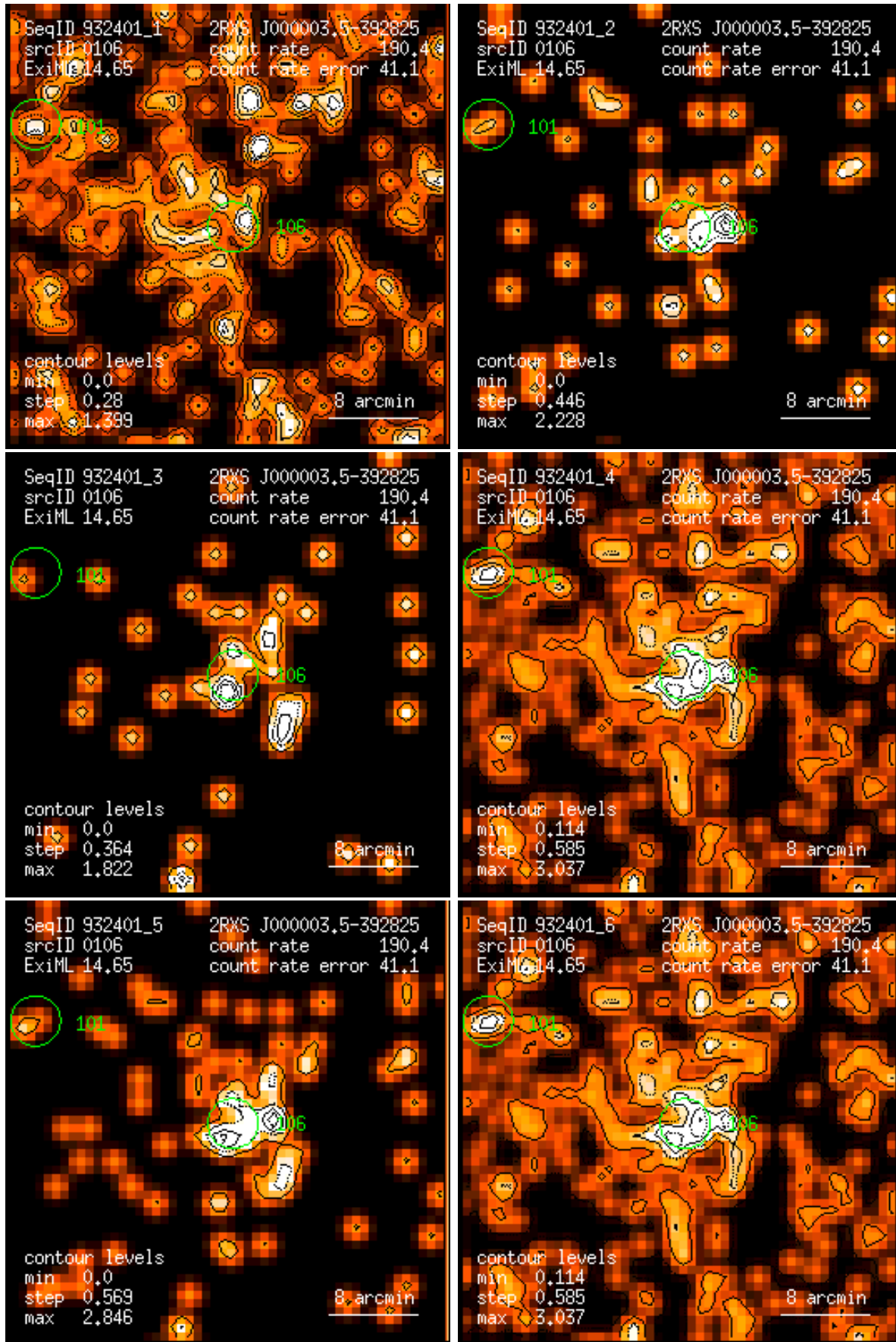
Figure 106: RASS 932401: detection 0106: band rate images, Gaussian filter: (1) PSPC channels 11 – 41, (2) 52 – 90, (3) 91 – 201, (4) 11 – 235, (5) 52 – 201, (6) 11 – 201. Broad band rates in counts/ks. Band rate contour levels in counts/ks/arcmin 2 .
