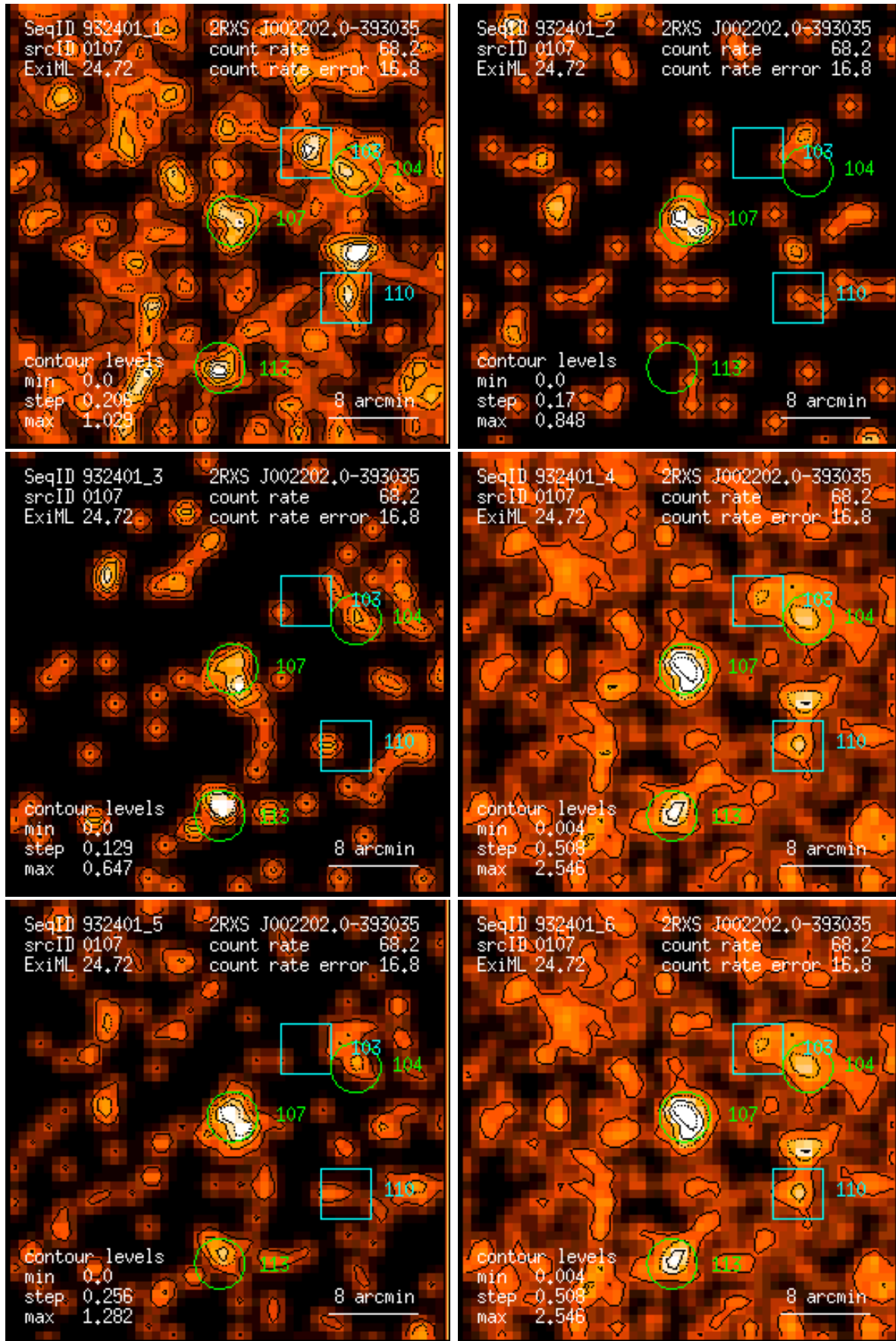
Figure 107: RASS 932401: detection 0107: band rate images, Gaussian filter: (1) PSPC channels 11 – 41, (2) 52 – 90, (3) 91 – 201, (4) 11 – 235, (5) 52 – 201, (6) 11 – 201. Broad band rates in counts/ks. Band rate contour levels in counts/ks/arcmin 2 .
