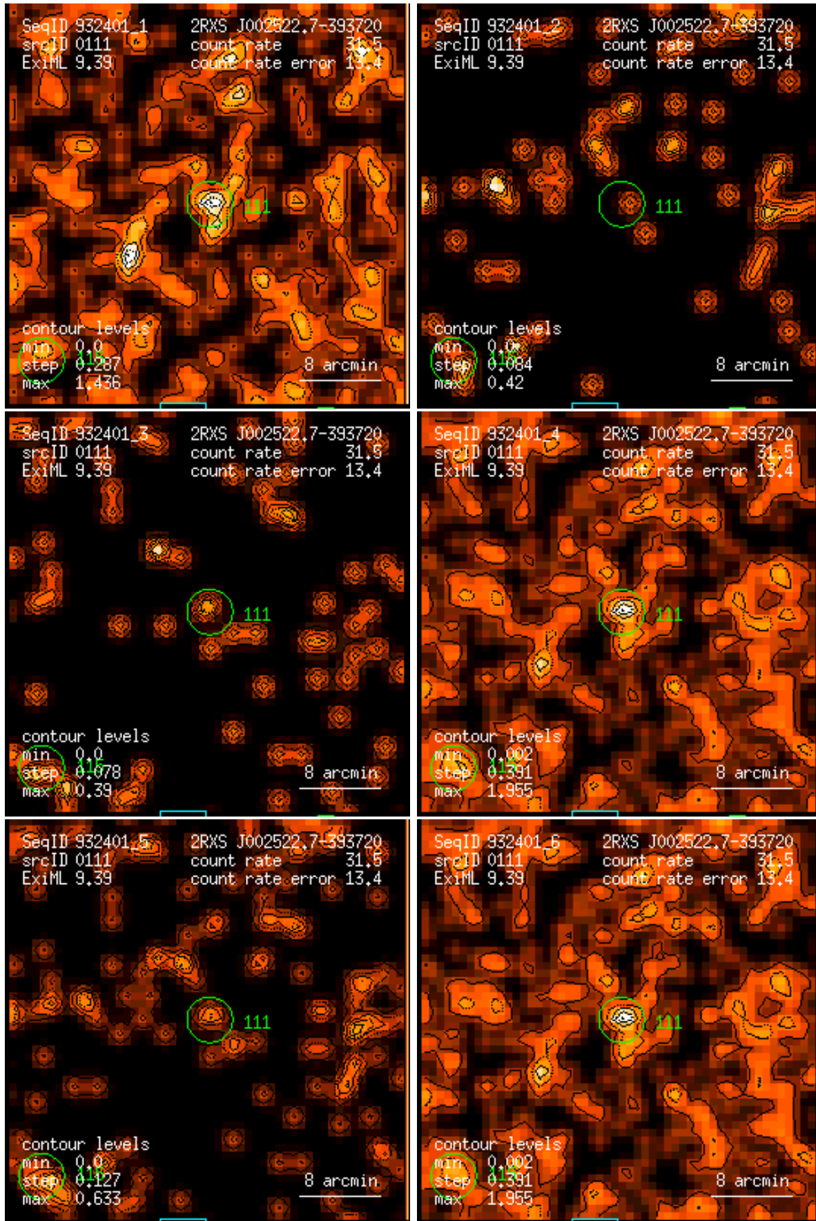
Figure 111: RASS 932401: detection 0111: band rate images, Gaussian filter: (1) PSPC channels 11 – 41, (2) 52 – 90, (3) 91 – 201, (4) 11 – 235, (5) 52 – 201, (6) 11 – 201. Broad band rates in counts/ks. Band rate contour levels in counts/ks/arcmin 2 .
