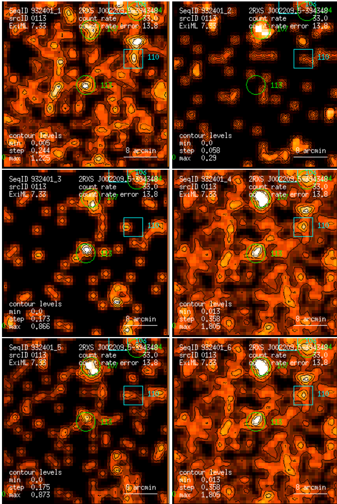
Figure 113: RASS 932401: detection 0113: band rate images, Gaussian filter: (1) PSPC channels 11 – 41, (2) 52 – 90, (3) 91 – 201, (4) 11 – 235, (5) 52 – 201, (6) 11 – 201. Broad band rates in counts/ks. Band rate contour levels in counts/ks/arcmin 2 .
