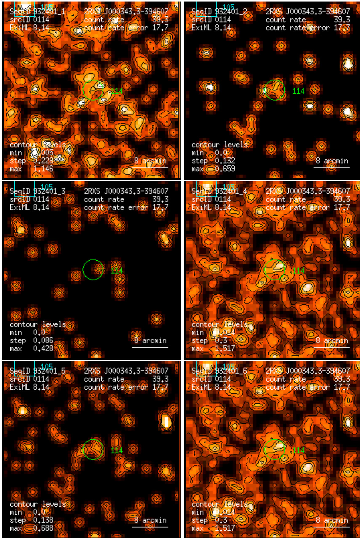
Figure 114: RASS 932401: detection 0114: band rate images, Gaussian filter: (1) PSPC channels 11 – 41, (2) 52 – 90, (3) 91 – 201, (4) 11 – 235, (5) 52 – 201, (6) 11 – 201. Broad band rates in counts/ks. Band rate contour levels in counts/ks/arcmin 2 .
