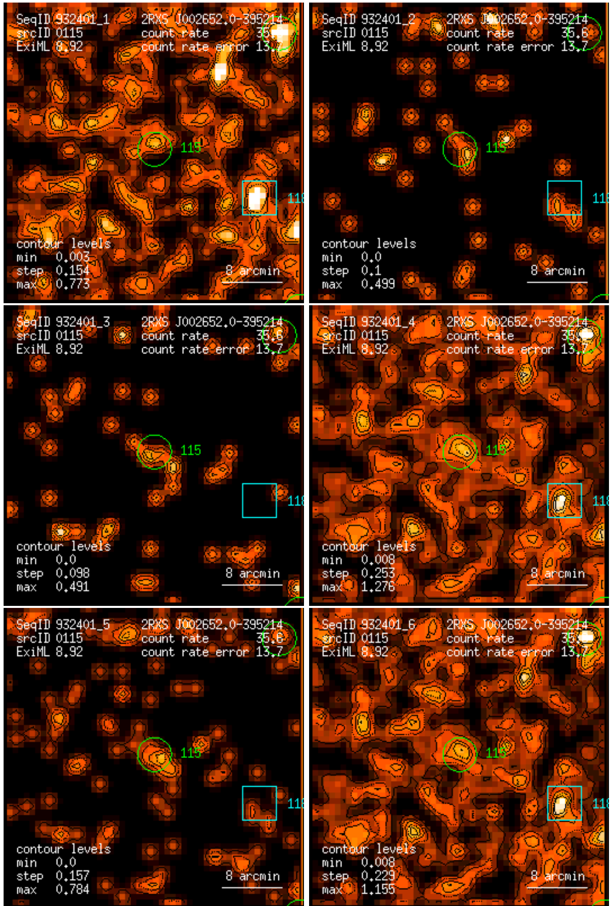
Figure 115: RASS 932401: detection 0115: band rate images, Gaussian filter: (1) PSPC channels 11 – 41, (2) 52 – 90, (3) 91 – 201, (4) 11 – 235, (5) 52 – 201, (6) 11 – 201. Broad band rates in counts/ks. Band rate contour levels in counts/ks/arcmin 2 .
