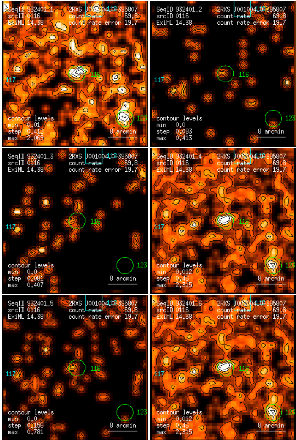
Figure 116: RASS 932401: detection 0116: band rate images, Gaussian filter: (1) PSPC channels 11 – 41, (2) 52 – 90, (3) 91 – 201, (4) 11 – 235, (5) 52 – 201, (6) 11 – 201. Broad band rates in counts/ks. Band rate contour levels in counts/ks/arcmin 2 .
